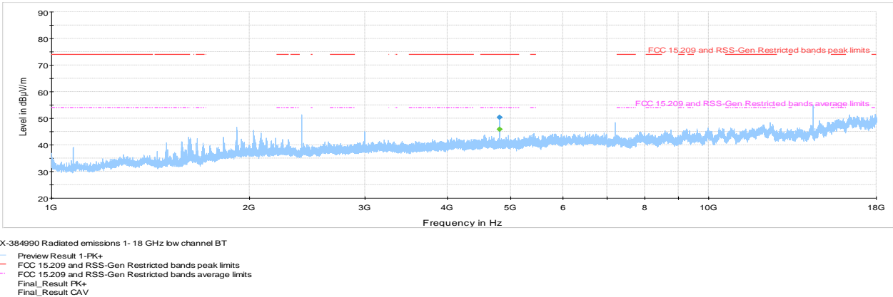
Figure 8.6-30: Radiated spurious emissions within 1-18 GHz, low channel
