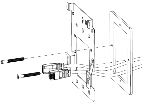
Figure 7 Mounting Plate to Gang Box(1)
