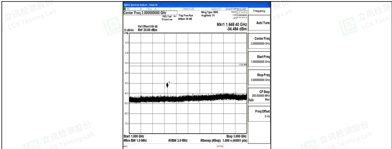
Band5_3MHz_16QAM_20415_1RB#0_1000~3000_1000~3000
