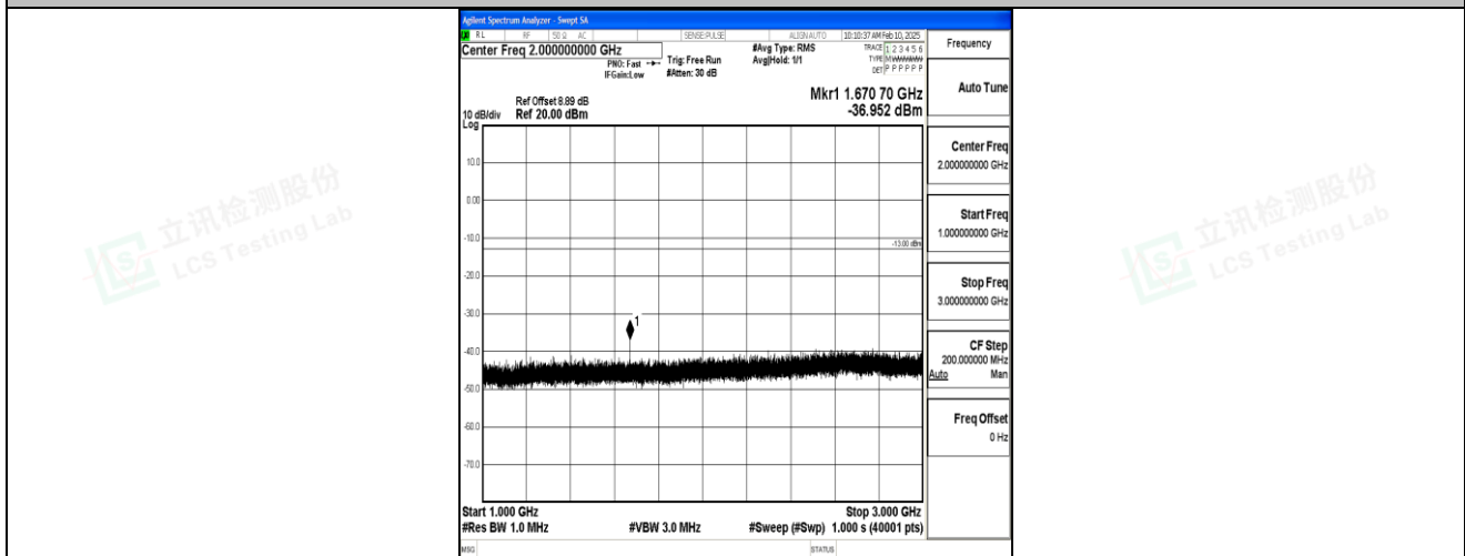
Band5_3MHz_QPSK_20525_1RB#0_1000~3000_1000~3000
