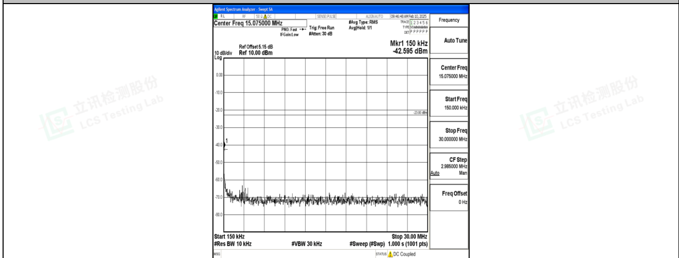
Band5_1.4MHz_16QAM_20525_1RB#0_0.15~30_0.15~30
