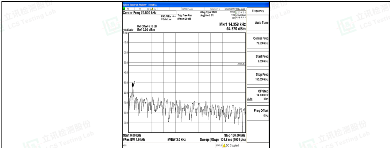
Band5_3MHz_16QAM_20415_1RB#0_0.009~0.15_0.009~0.15
