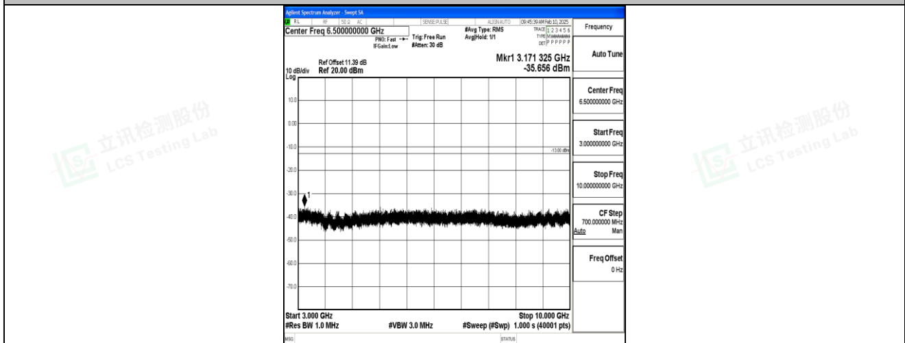
Band5_1.4MHz_QPSK_20407_1RB#0_3000~10000_3000~10000
