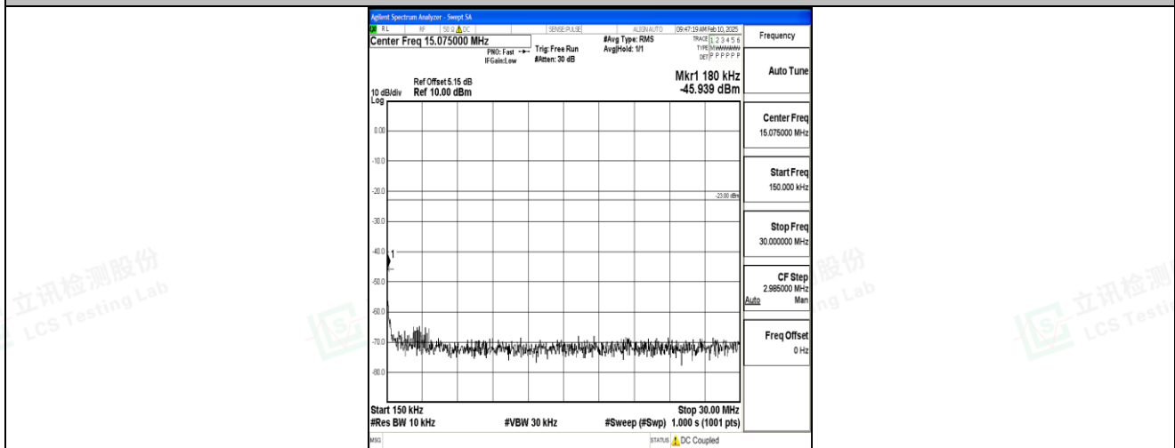
Band5_1.4MHz_QPSK_20643_1RB#0_0.15~30_0.15~30
