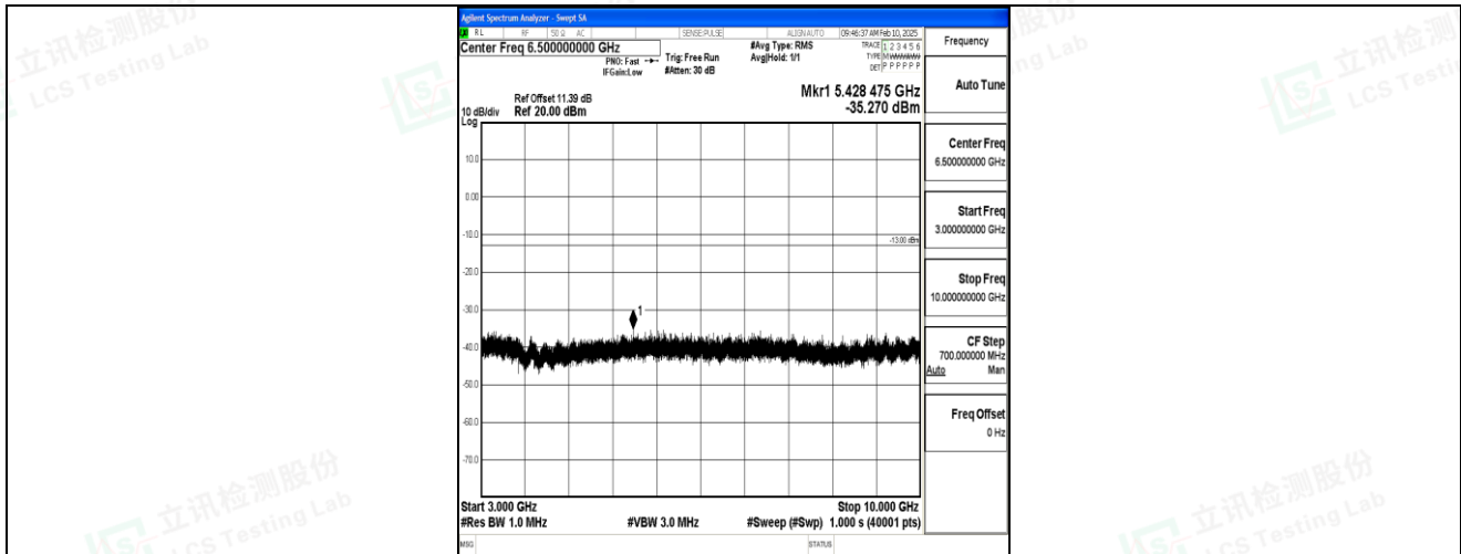
Band5_1.4MHz_QPSK_20525_1RB#0_3000~10000_3000~10000
