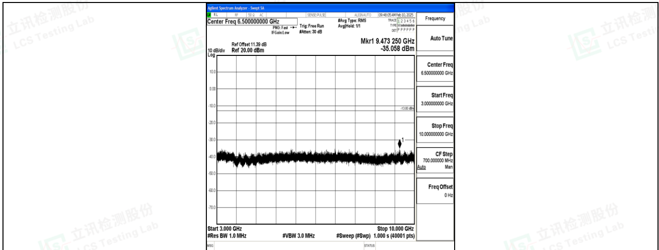
Band5_1.4MHz_16QAM_20643_1RB#0_3000~10000_3000~10000
