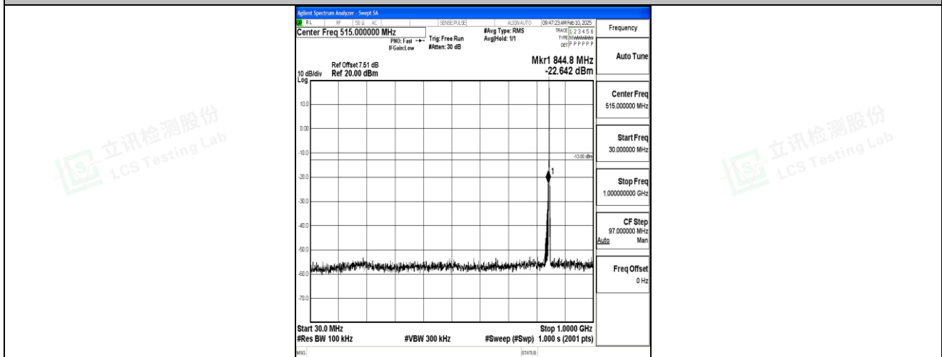
Band5_1.4MHz_QPSK_20643_1RB#0_30~1000_30~1000
