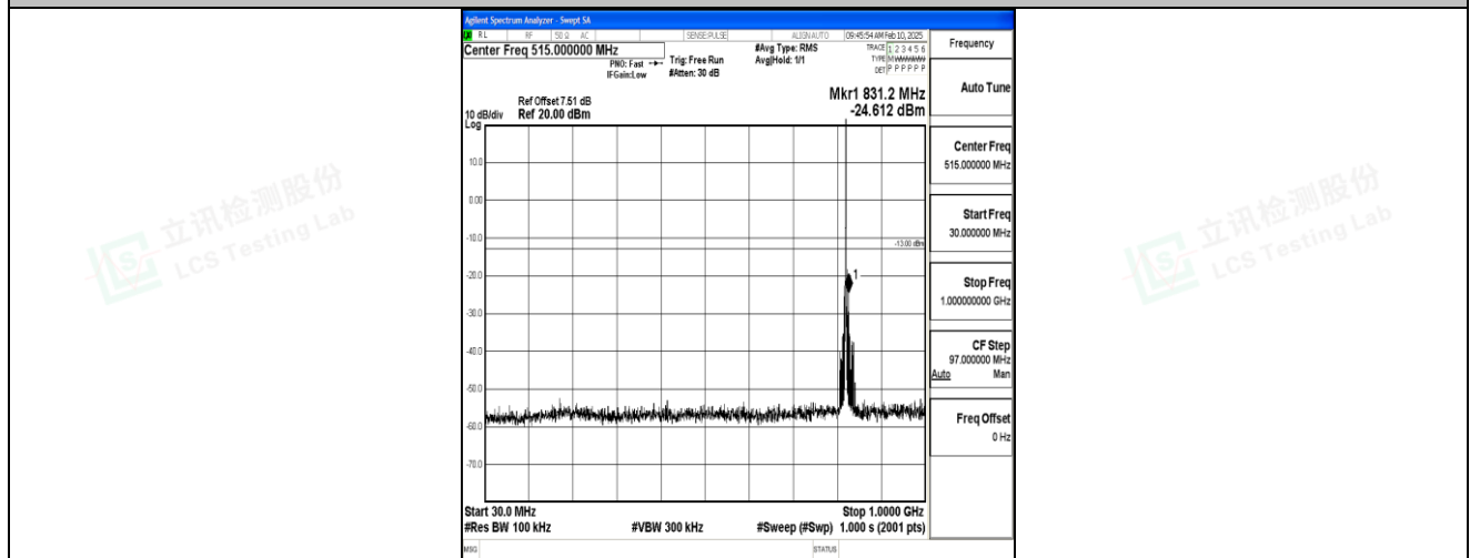
Band5_1.4MHz_16QAM_20407_1RB#0_30~1000_30~1000
