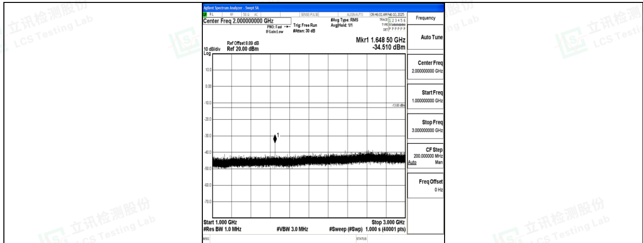
Band5_1.4MHz_16QAM_20407_1RB#0_1000~3000_1000~3000
