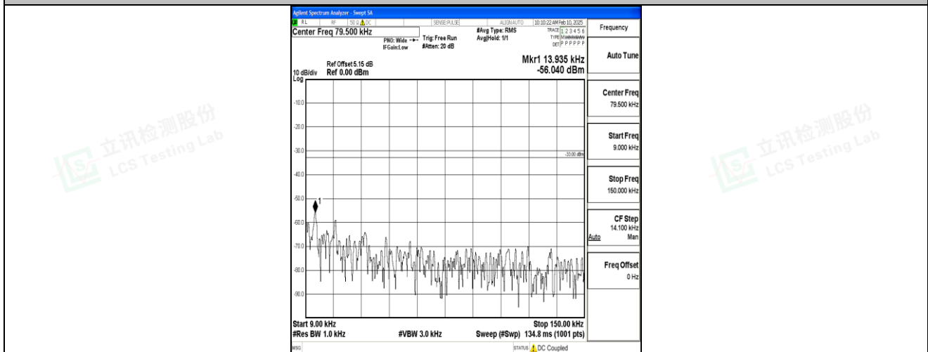
Band5_3MHz_QPSK_20525_1RB#0_0.009~0.15_0.009~0.15
