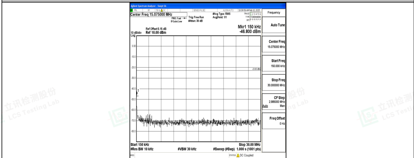
Band5_3MHz_16QAM_20415_1RB#0_0.15~30_0.15~30
