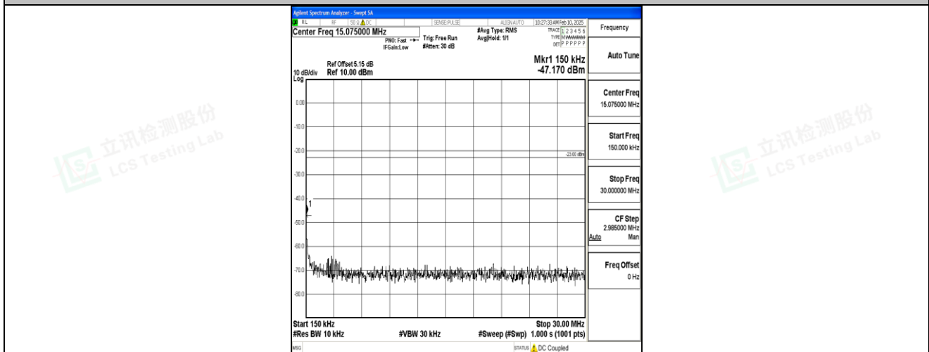
Band5_5MHz_QPSK_20425_1RB#0_0.15~30_0.15~30
