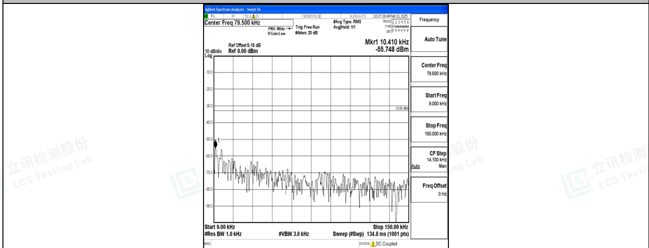
Band5_5MHz_QPSK_20425_1RB#0_0.009~0.15_0.009~0.15
