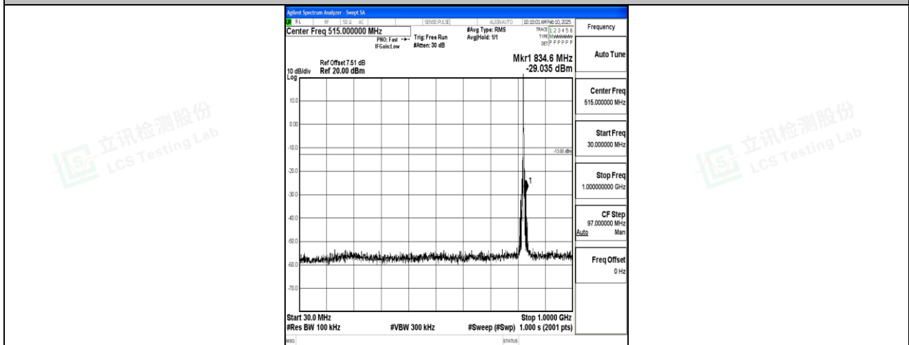
Band5_3MHz_16QAM_20415_1RB#0_30~1000_30~1000
