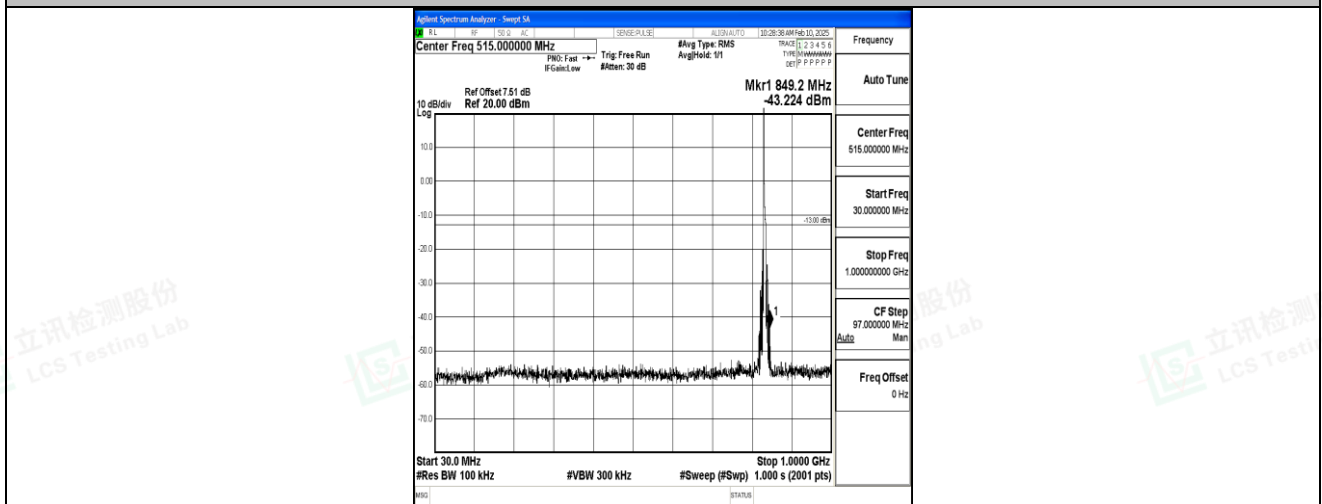
Band5_5MHz_QPSK_20525_1RB#0_30~1000_30~1000
