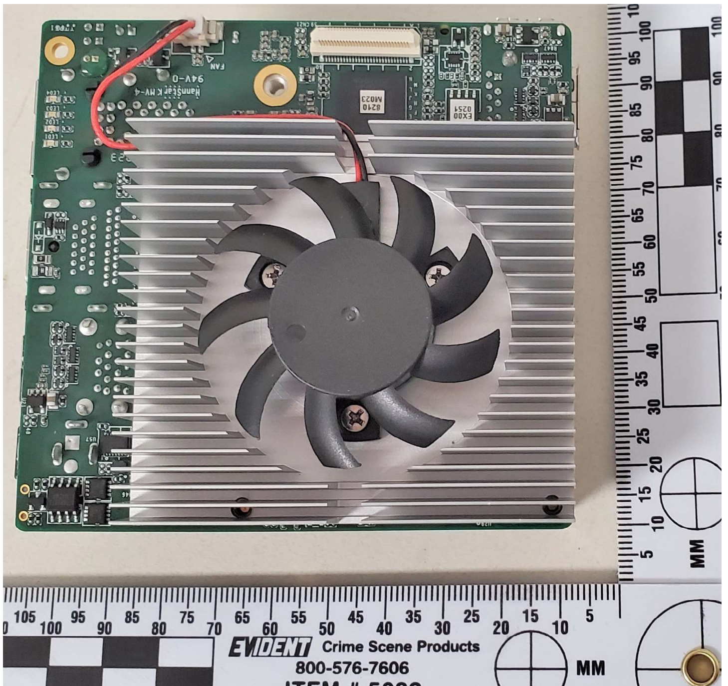
PC Board Bottom Side
