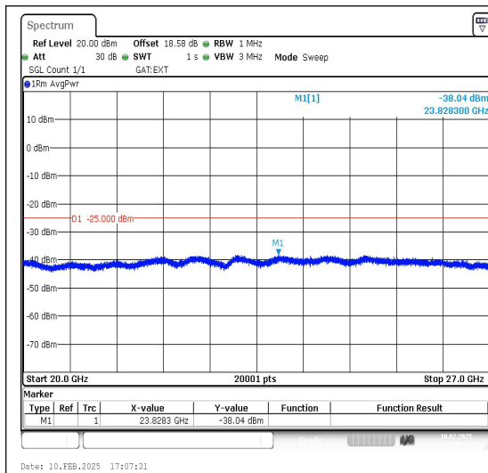
Band41_20MHz_QPSK_41490_1RB#0_20000~27000
