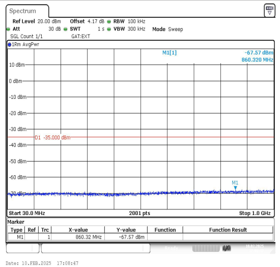
Band41_20MHz_16QAM_41490_1RB#0_30~1000
