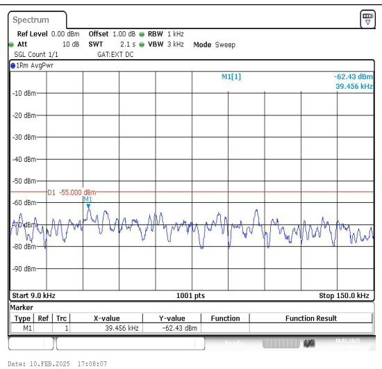
Band41_20MHz_16QAM_41490_1RB#0_0.009~0.15
