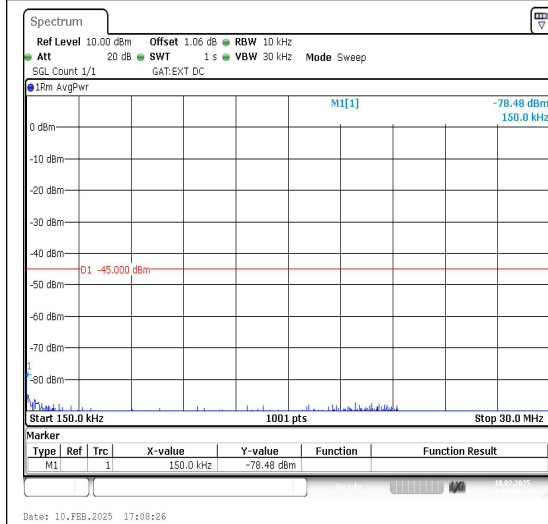
Band41_20MHz_16QAM_41490_1RB#0_0.15~3
