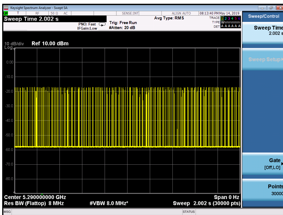
EUT data traffic (5290MHz)
