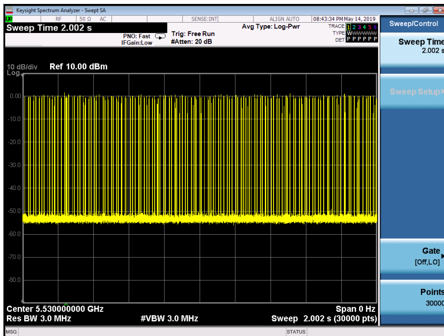
EUT data traffic (5530MHz)
