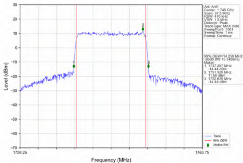
n66_15kHz_SISO_NTNV_15MHz_CP-OFDM_16 QAM_1745MHz_Outer_Full
