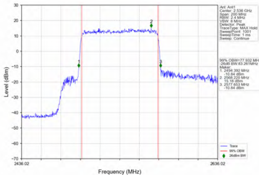
n41_30kHz_SISO_NTNV_80MHz_CP-OFDM QPSK_2536.02MHz_Outer_Full
