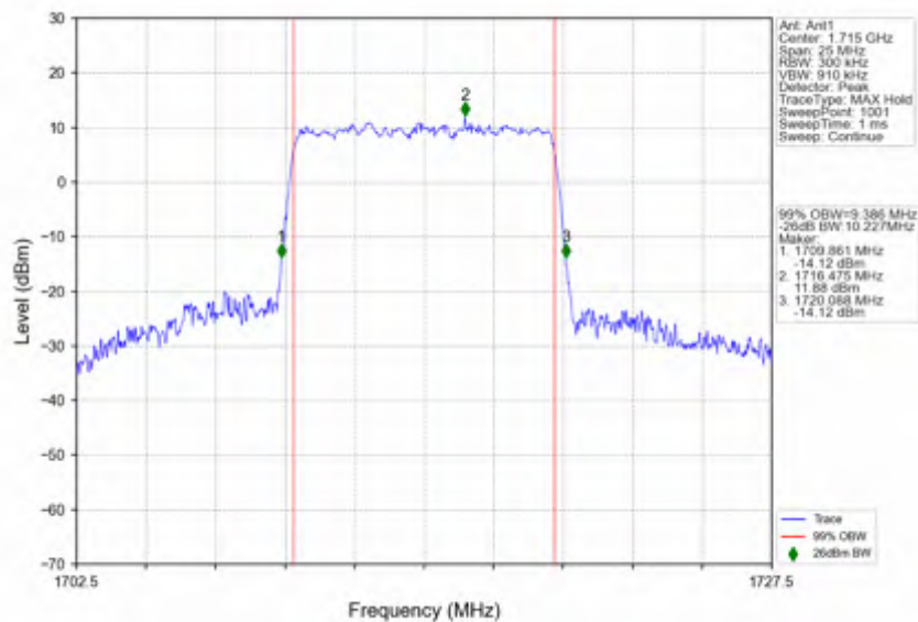
n66_15kHz_SISO_NTV_10MHz_CP-OFDM_QPSK_1715MHz_Outer_Full
