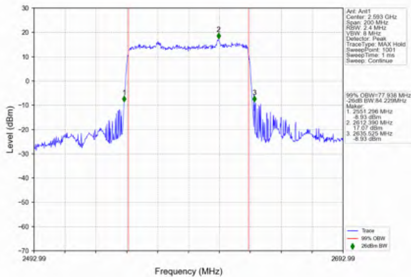
n41_30kHz_SISO_NTNV_80MHz_DFT-s-OFDM_PI/2_BPSK_2592.99MHz_Outer_Full
