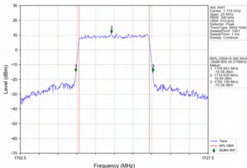
n66 15kHz SISO NTNV 10MHz CP-OFDM 64 QAM 1715MHz Outer Full
