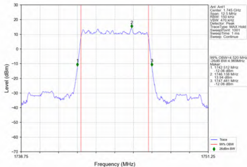
n66_15kHz_SISO_NTNV_5MHz_DFT-s-OFDM_PI/2_BPSK_1745MHz_Outer_Full
