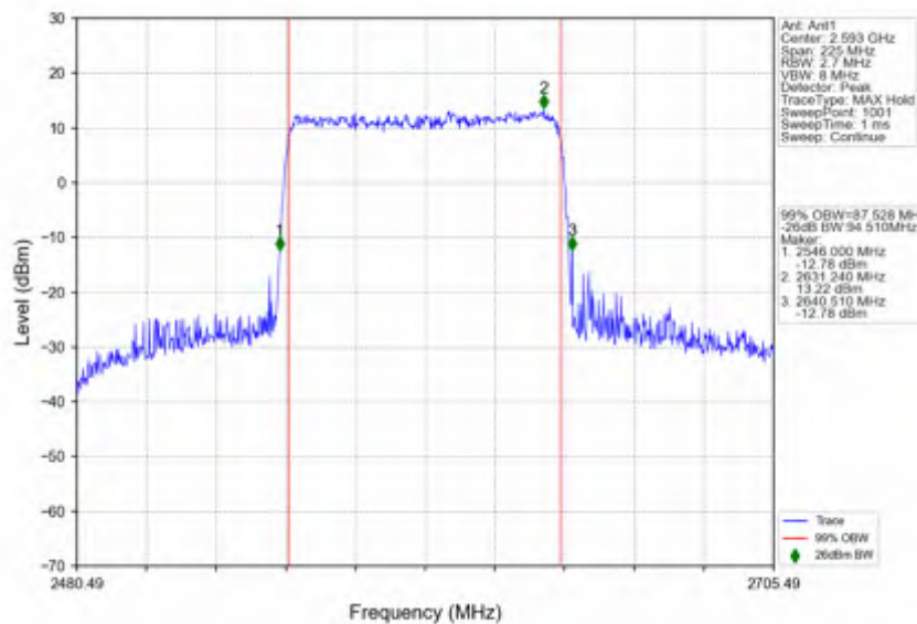
n41_30kHz_SISO_NTNV_90MHz_DFT-s-OFDM_256_QAM_2592.99MHz_Outer_Full
