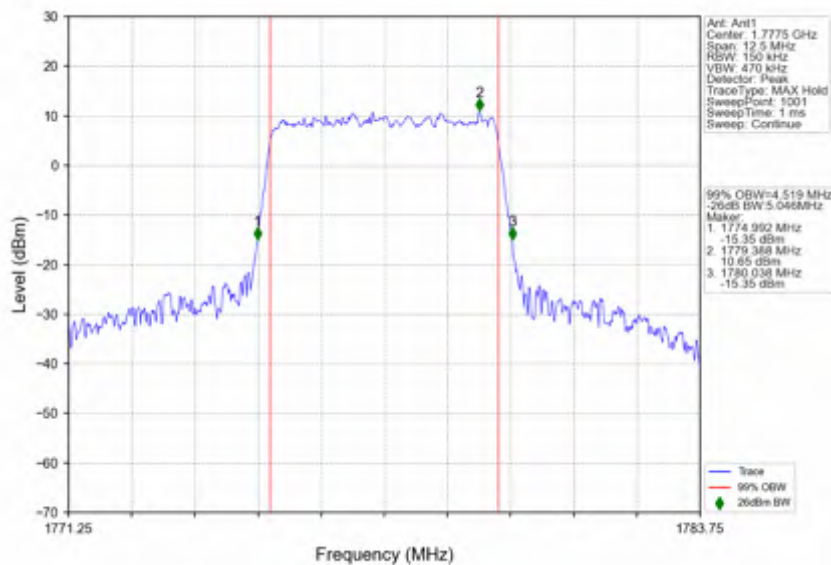
n66_15kHz_SISO_NTNV_5MHz_CP-OFDM 64 QAM_1777.5MHz_Outer_Full
