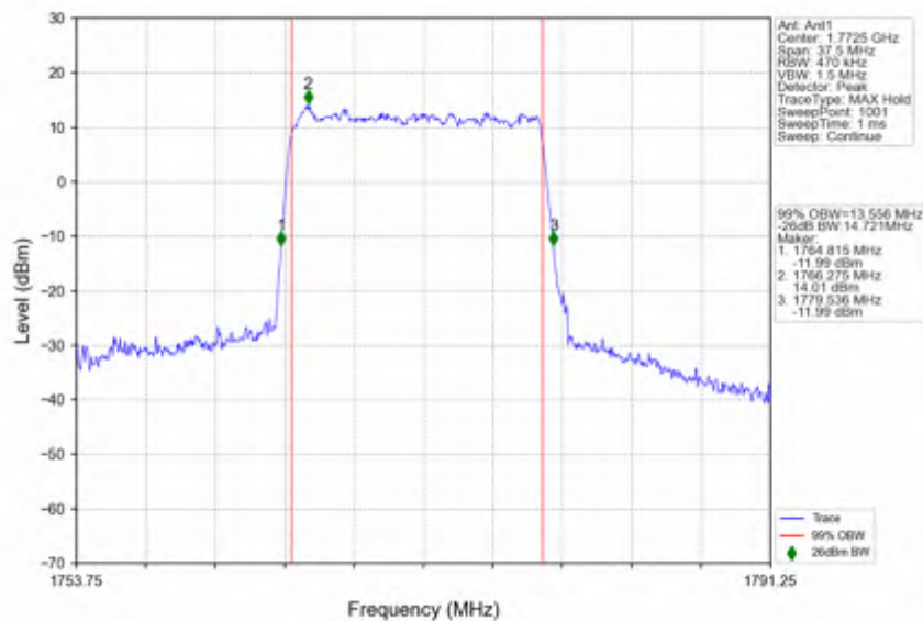
n66 15kHz SISO NTN 15MHz DFT-s-OFDM QPSK 1772.5MHz Outer Full
