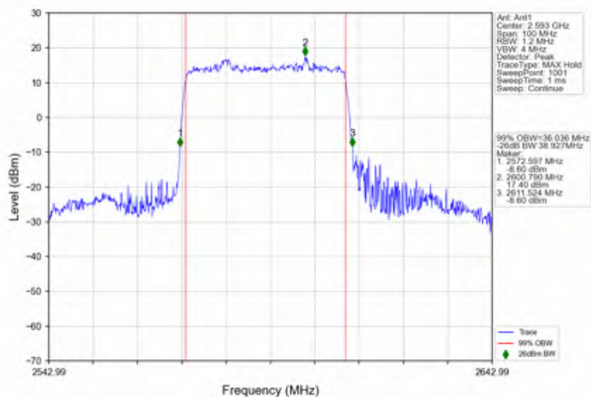
n41_30kHz_SISO_NTNV_40MHz_DFT-s-OFDM_PI/2_BPSK_2592.99MHz_Outer_Full
