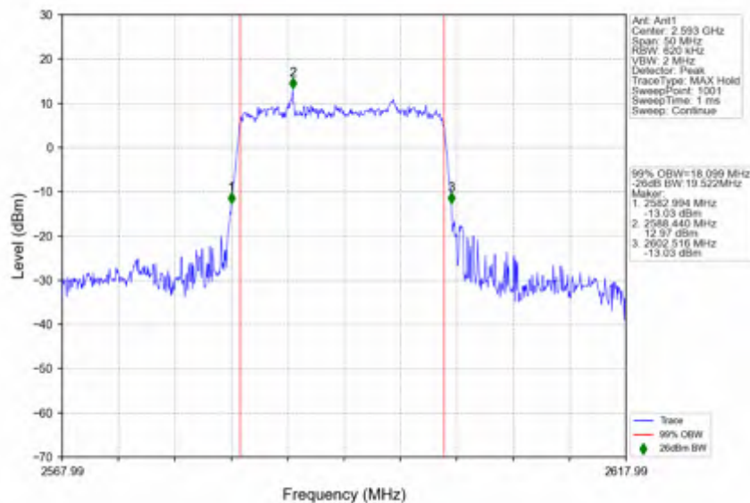
n41_30kHz_SISO_NTNV_20MHz_DFT-s-OFDM_PI/2_BPSK_2592.99MHz_Outer_Full
