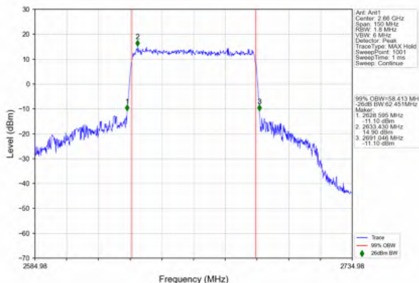
n41 30kHz SISO NTNV 60MHz CP-OFDM QPSK 2659.98MHz Outer Full
