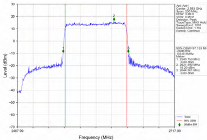
n41_30kHz_SISO_NTNV_100MHz_DFT-s-OFDM_16_QAM_2592.99MHz_Outer_Full
