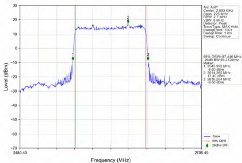
n41_30kHz_SISO_NTNV_90MHz_DFT-s-OFDM_PI/2_BPSK_2592.99MHz_Outer_Full
