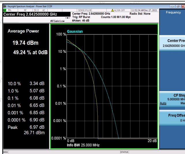
Band41-5MHz-QPSK-41115-25RB#0
