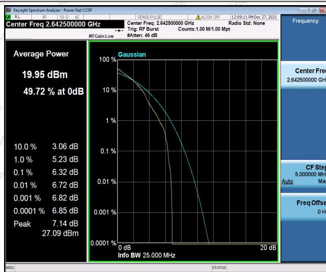
Band41-10MHz-QPSK-41115-50RB#0
