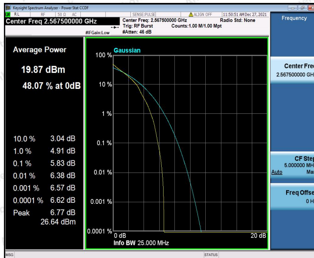
Band41-5MHz-QPSK-40365-25RB#0
