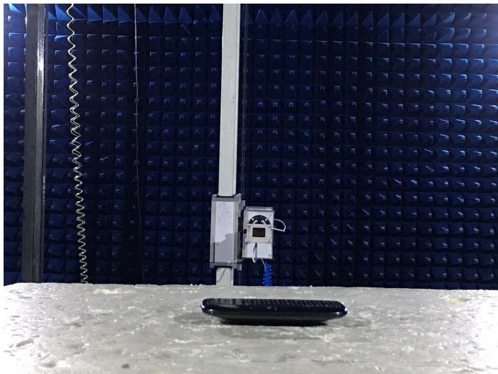
Photograph 4: Set-up for Radiated Spurious Emission (18GHz ~ 26GHz)
