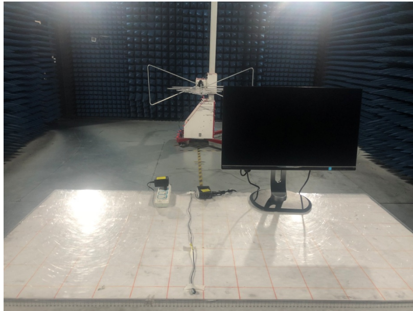
Model No.: Centro-8M Radiated Emission
