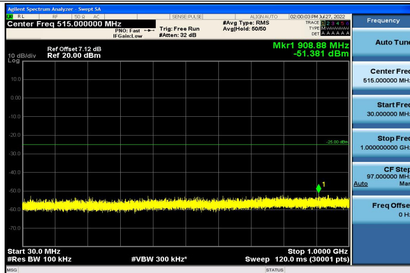
Band7-5MHz-QPSK-21100-1RB#0-30~1000MHz
