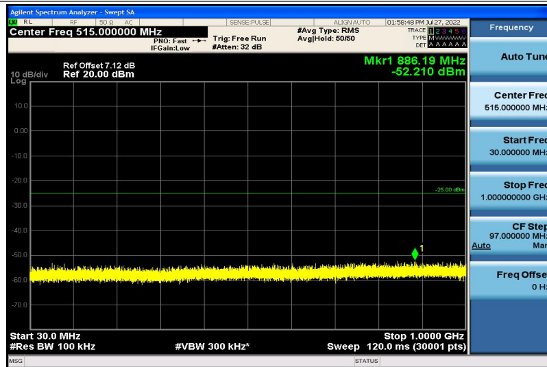
Band7-5MHz-QPSK-20775-1RB#0-30~1000MHz
