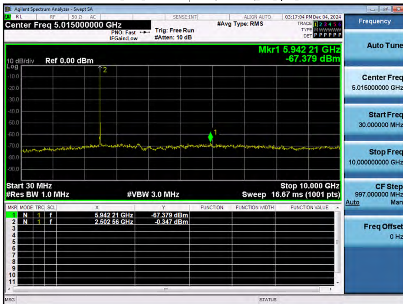
LTE B7_15 M_Conducted Spurious(30 M-10 G)_Low_QPSK_1RB
