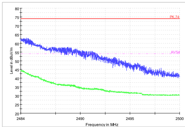
Radiated Emission Band Edge Channel No.:11 Test Mode: 802.11g Polarization: H
