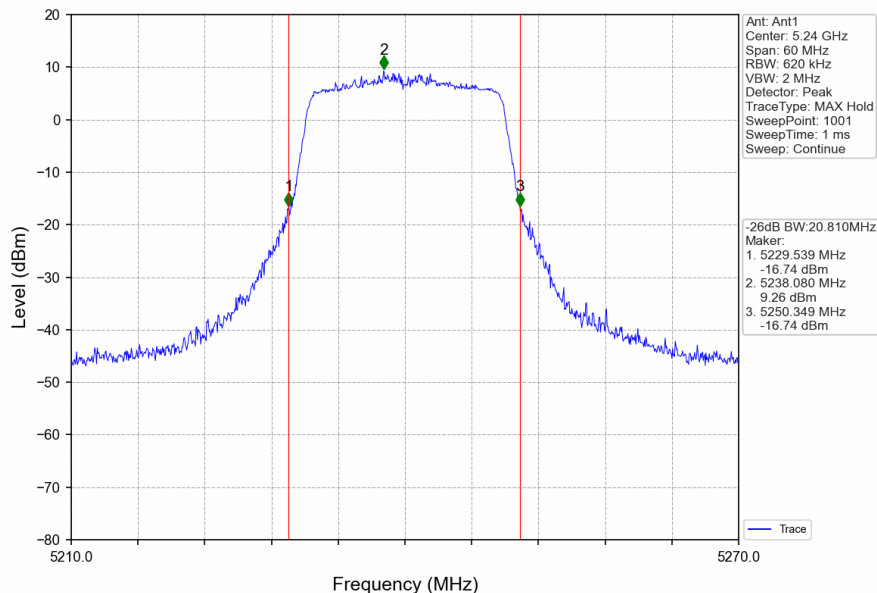
802.11ac(VHT20)_HCH_5240MHz_Ant1_NTNV
