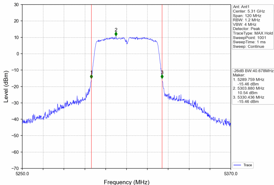
802.11ac(VHT40)_HCH_5310MHz_Ant1_NTNV
