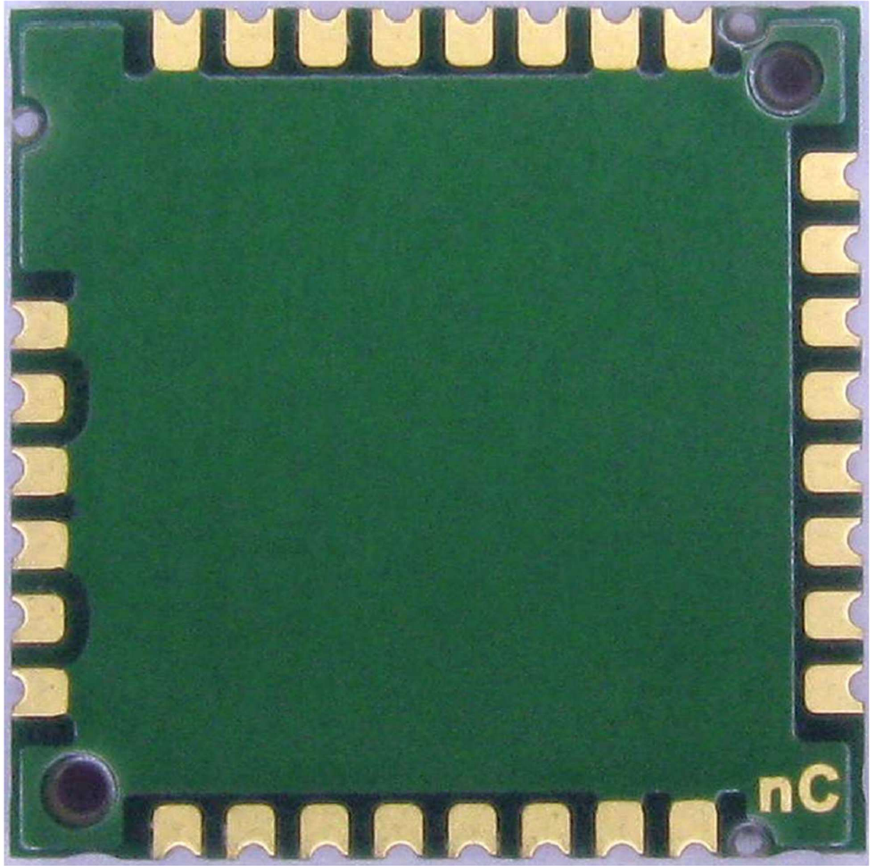
WIFI WIBEAR11N-SF1 module bottom view
