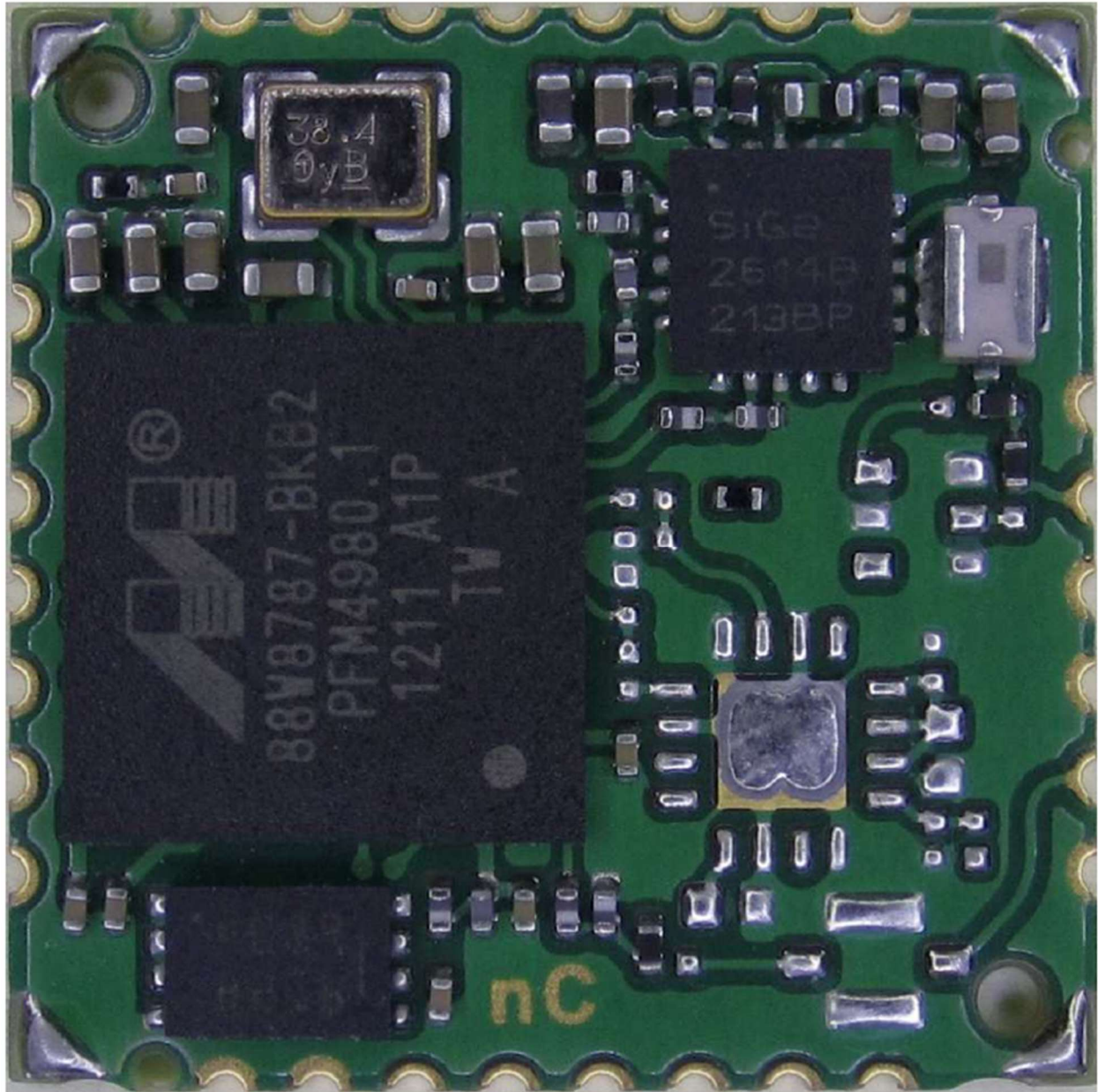
WIFI WIBEAR11N-SF1 module top view
