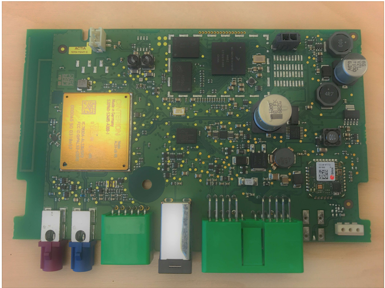
TEM4G top view
