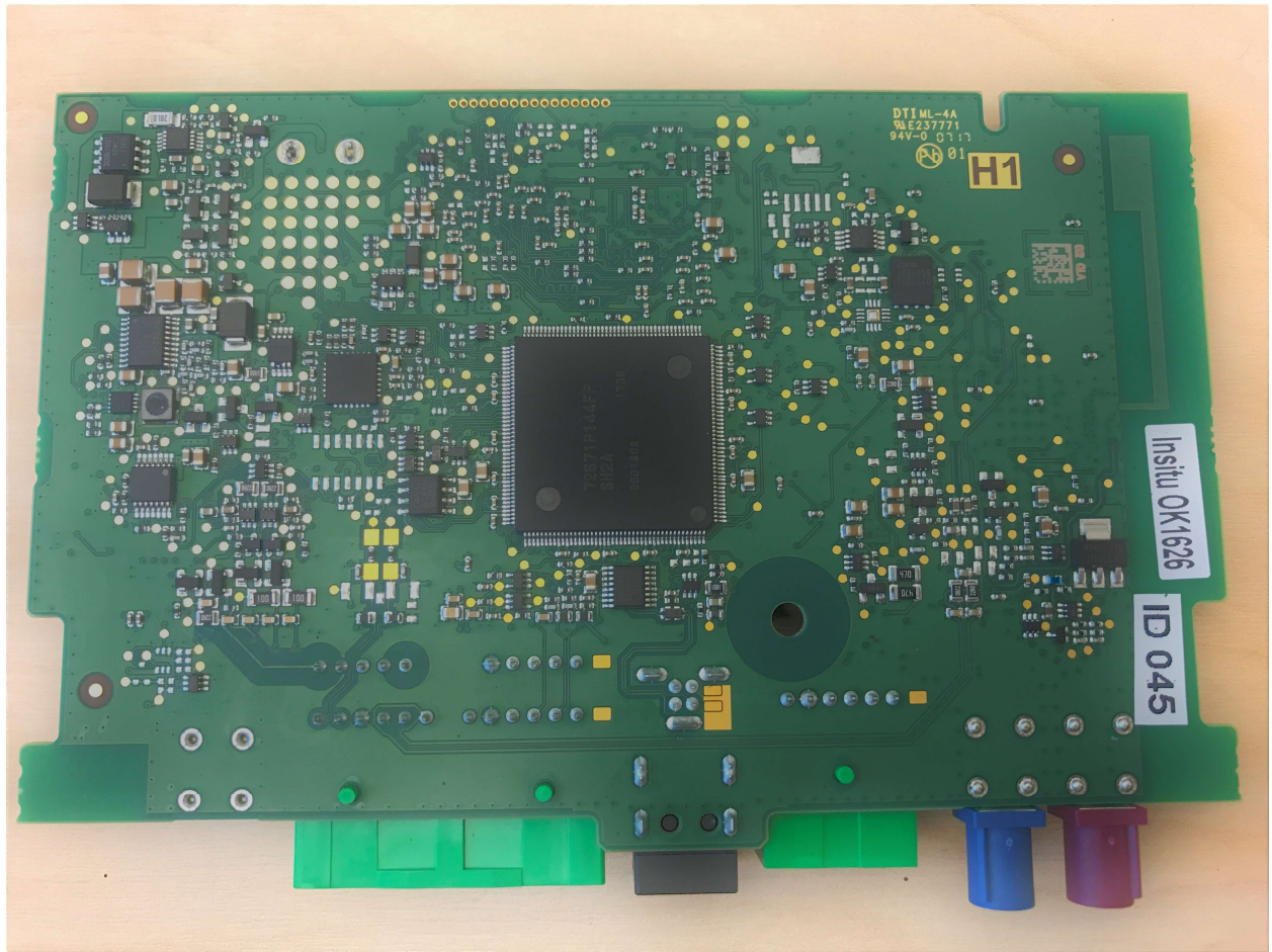
TEM4G bottom view
