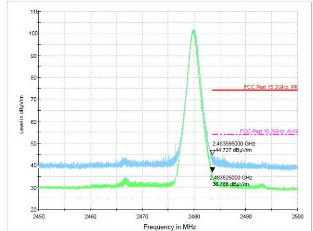
Test Mode: \pi/4 DQPSK-High
