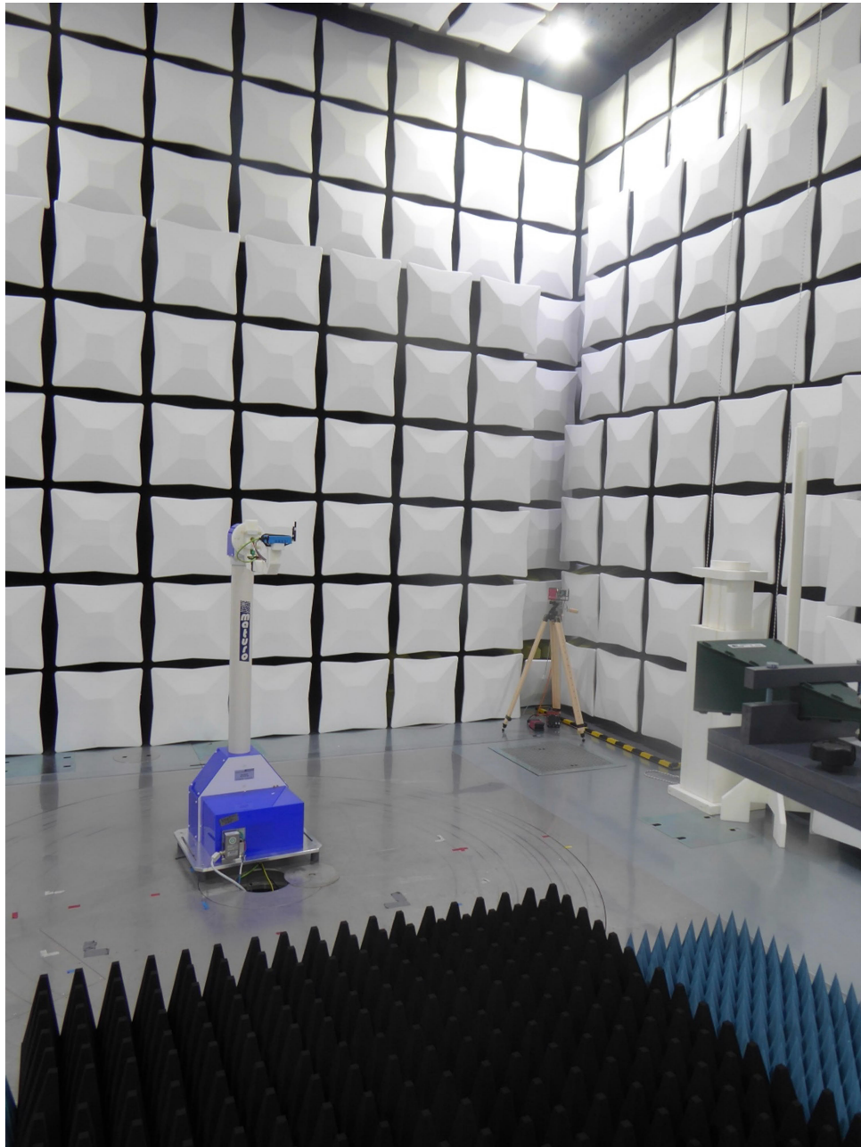
Test setup semi anechoic chamber M276, 12 GHz - 18 GHz
