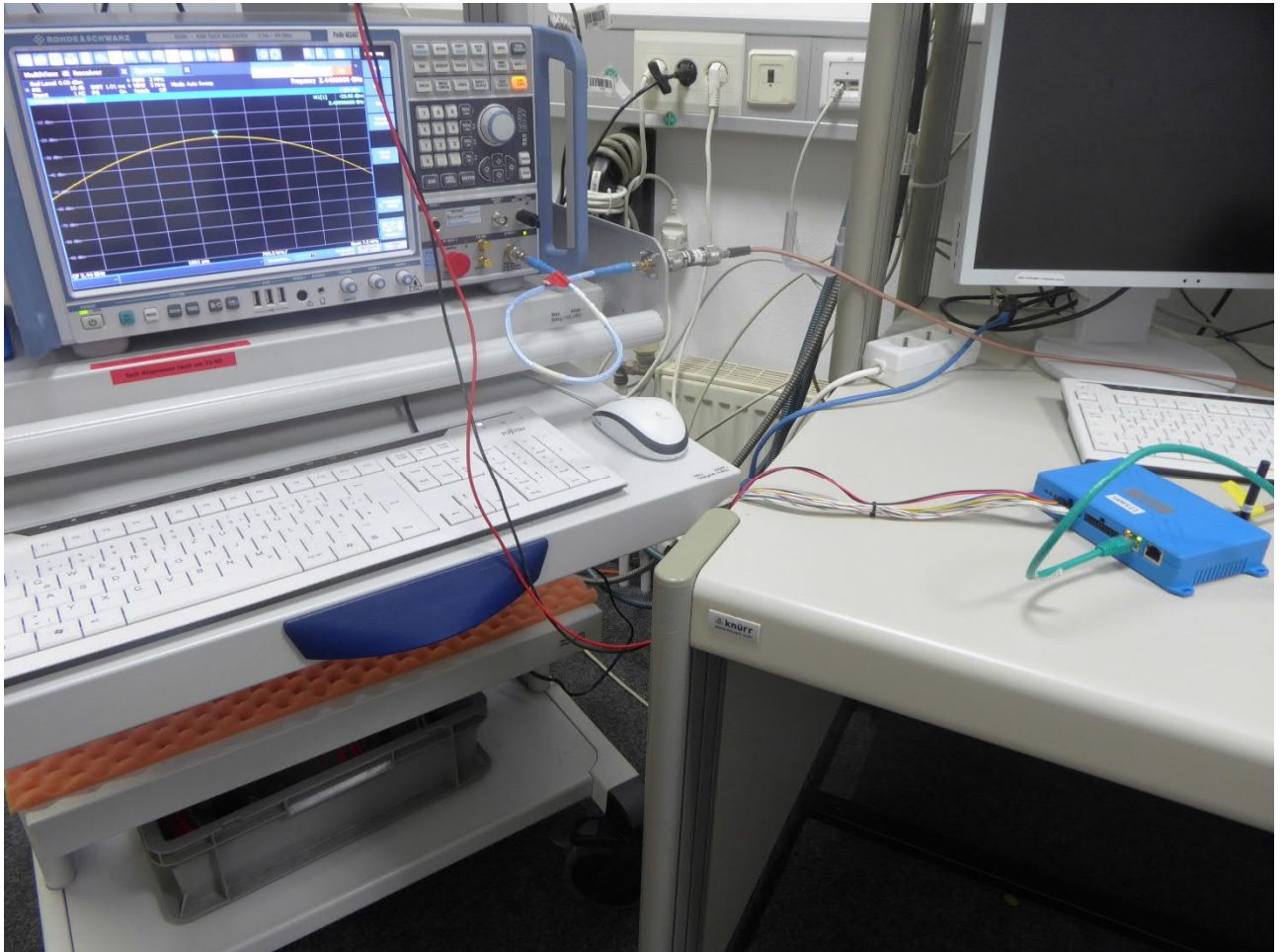
Test setup RF power measurements
