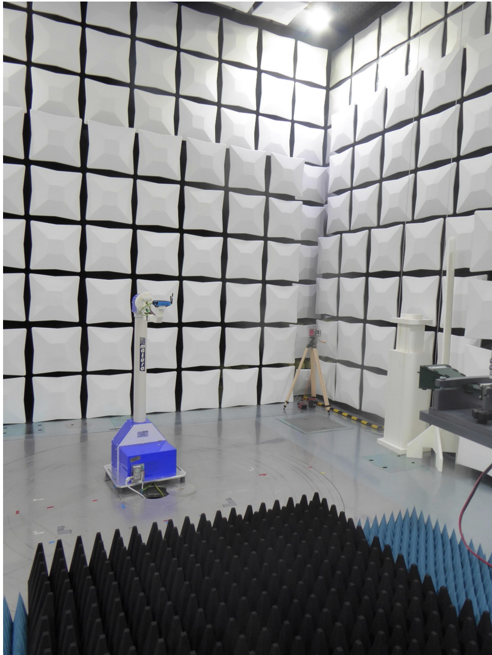
Test setup semi anechoic chamber M276, 18 GHz – 26.5 GHz
