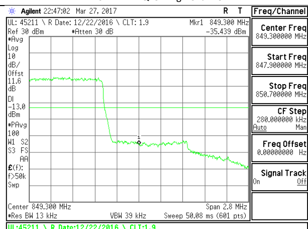
LTE B26 1.4MHz QPSK High Channel 1RB
