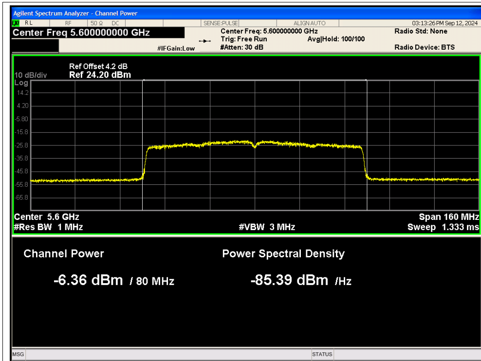
Power NVNT ac80 5600MHz Ant2
