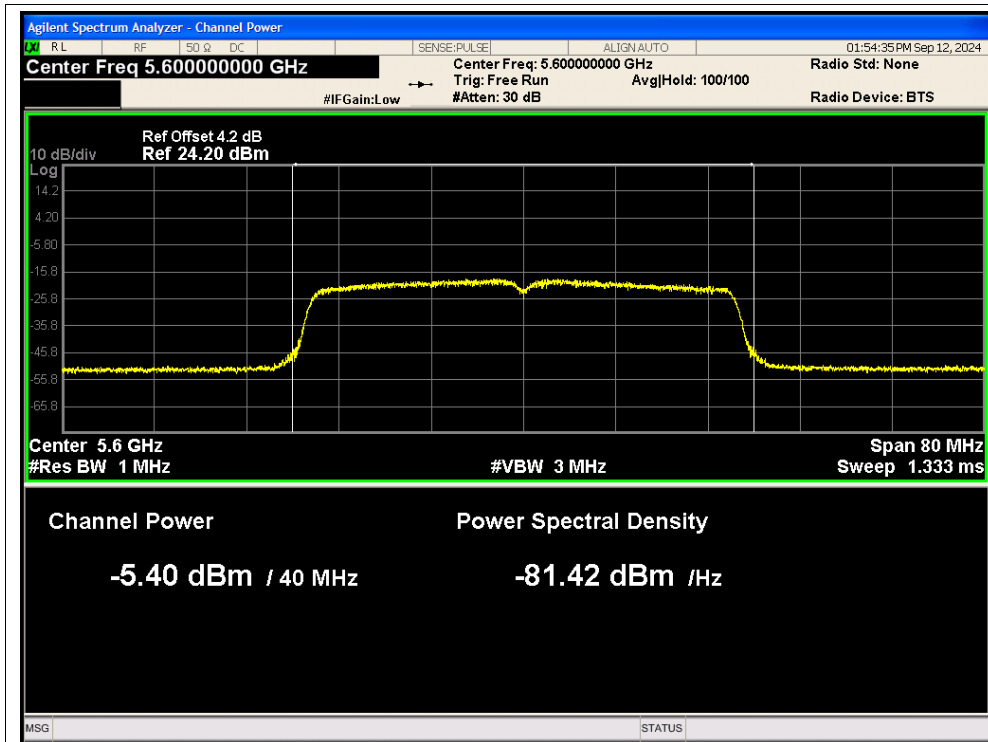
Power NVNT ac40 5600MHz Ant2
