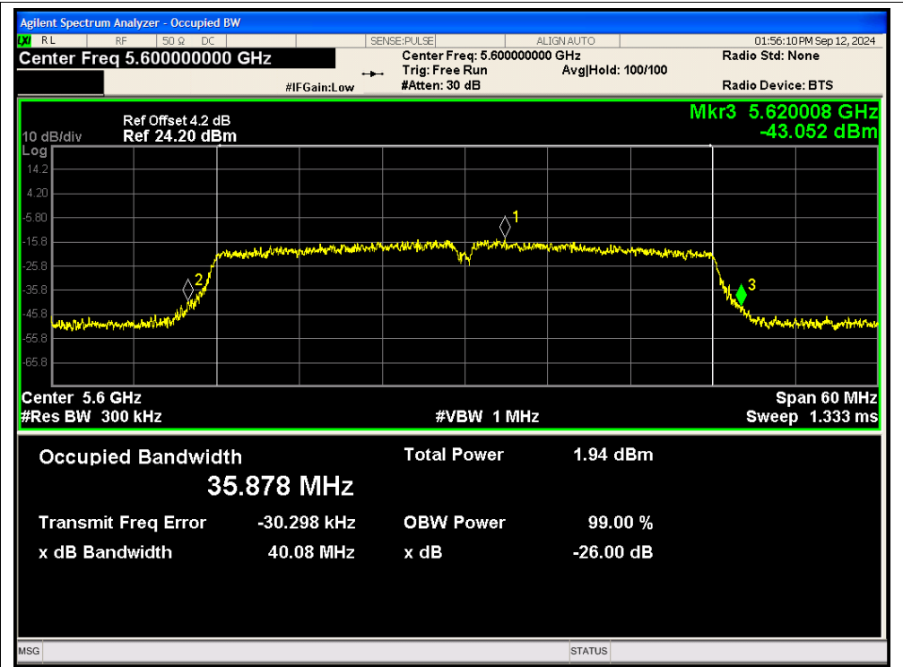
-26dB Bandwidth NVNT ac40 5600MHz Ant2
