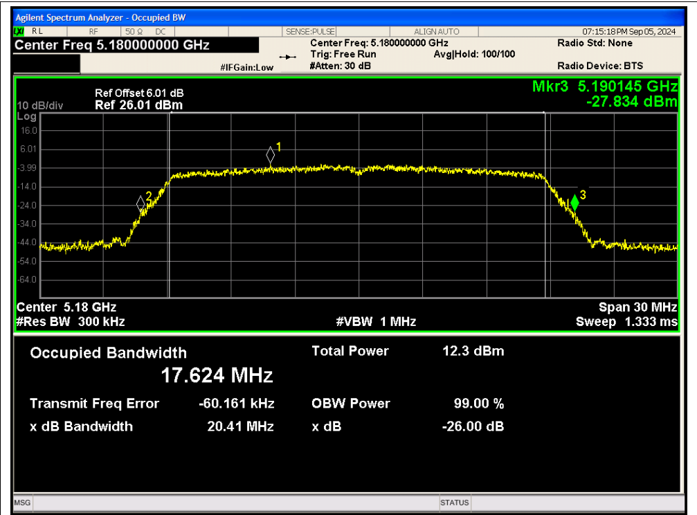
-26dB Bandwidth NVNT n20 5180MHz Ant2
