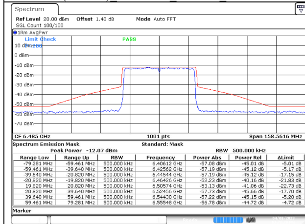
802.11ax (40MHz) 6485MHz Chain A NSS-1
