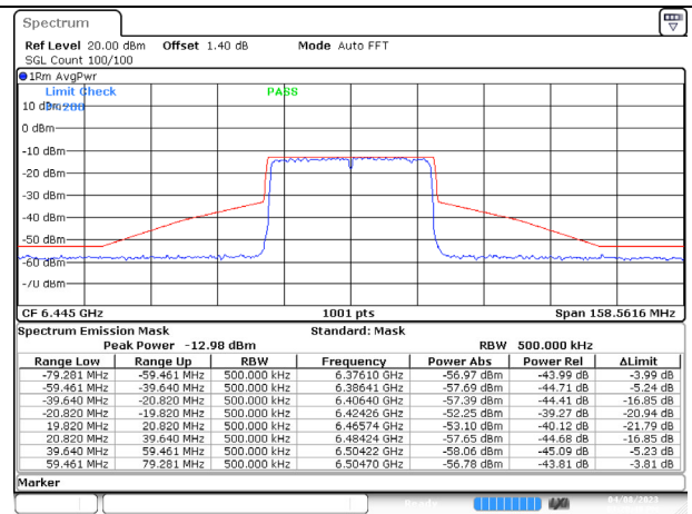
802.11ax (40MHz) 6445MHz Chain D NSS-1
