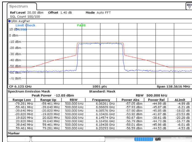
802.11ax (40MHz) 6125MHz Chain C NSS-1
