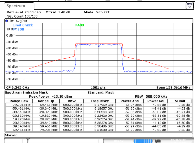
802.11ax (40MHz) 6245MHz Chain B NSS-1
