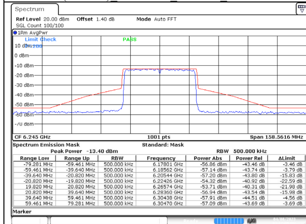
802.11ax (40MHz) 6245MHz Chain A NSS-1
