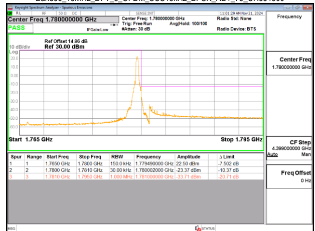
Band66_15MHz_DFT_s_OFDM_SCS15kHz_BPSK_RB1_78_CH354500
