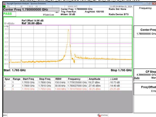
Band66_15MHz_CP_OFDM_SCS15kHz_QPSK_RB79_0_CH354500
