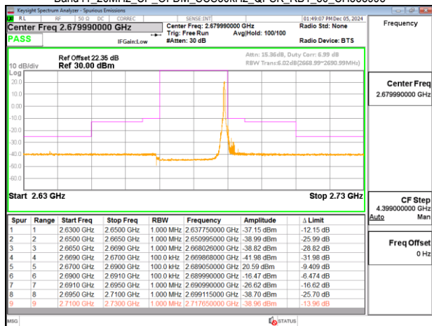
Band41_20MHz_CP_OFDM_SCS30kHz_QPSK_RB51_0_CH535998
