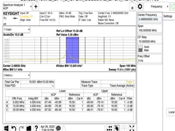
Band53_10MHz_DFT_s_OFDM_SCS30kHz_BPSK_RB1_0_CH497700
