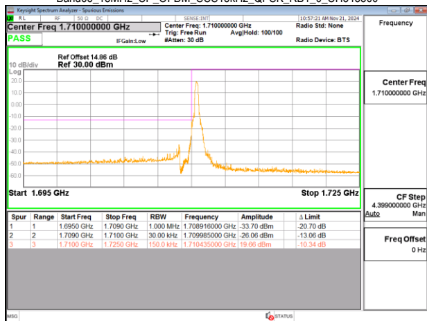
Band66_15MHz_CP_OFDM_SCS15kHz_QPSK_RB79_0_CH343500
