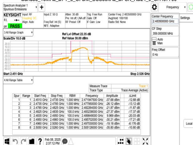
Band53_10MHz_DFT_s_OFDM_SCS30kHz_BPSK_RB1_0_CH497700
