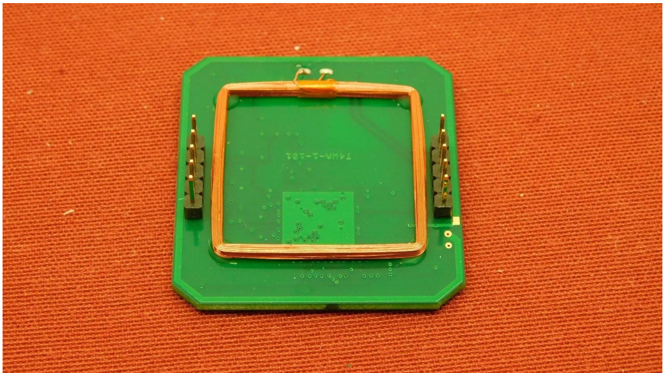
Picture 7: Bottom view of PCB, with loop antenna
