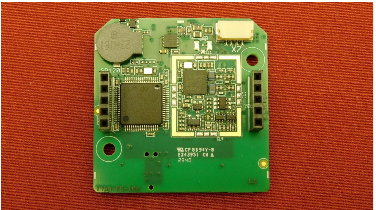
Picture 4: Top view of PCB with Processor
