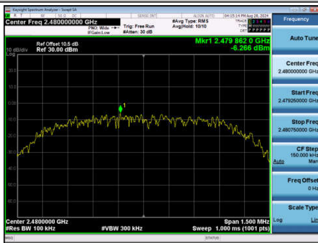
3DH5-Ant1-2480-0~Reference-PASS
