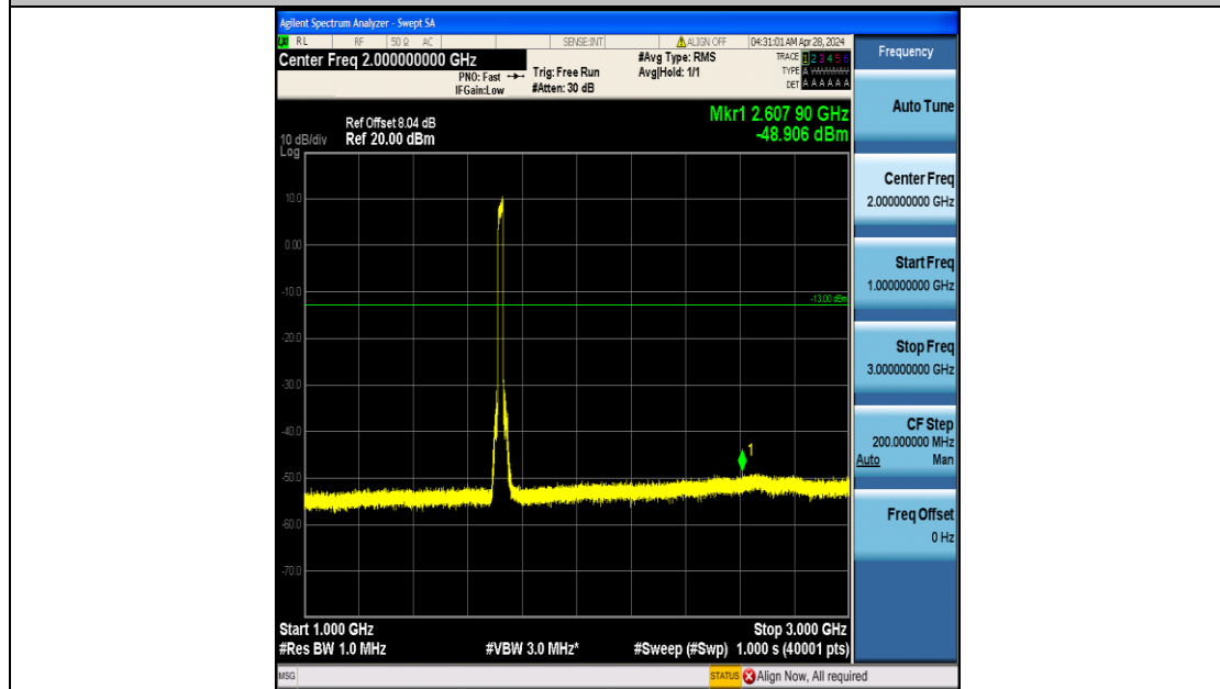
Band4_20MHz_16QAM_20050_100RB#0_1000~3000_1000~3000
