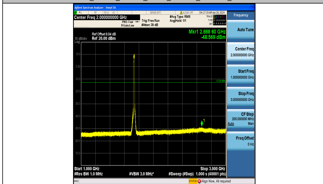
Band4_15MHz_16QAM_20175_75RB#0_1000~3000_1000~3000
