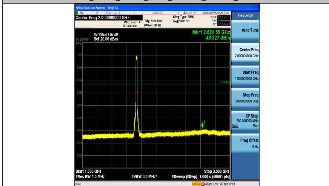
Band4_20MHz_16QAM_20175_100RB#0_1000~3000_1000~3000
