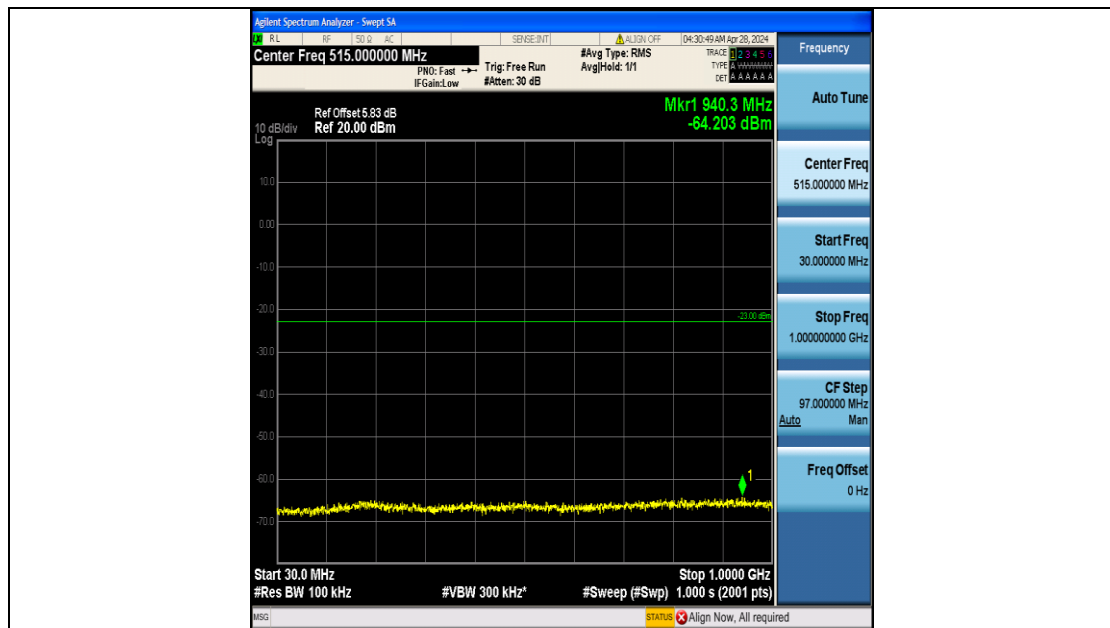
Band4_20MHz_16QAM_20050_100RB#0_30~1000_30~1000
