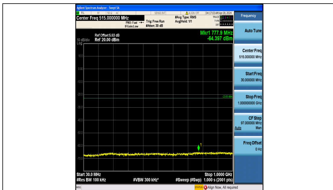
Band4_15MHz_16QAM_20175_75RB#0_30~1000_30~1000
