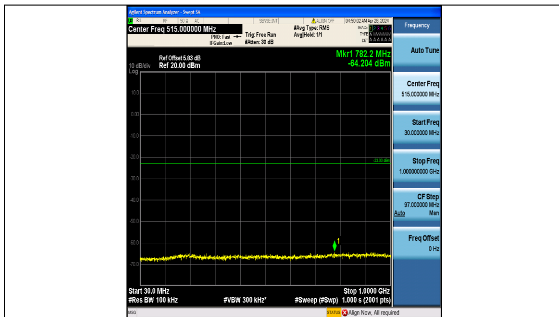
Band4_20MHz_16QAM_20175_100RB#0_30~1000_30~1000
