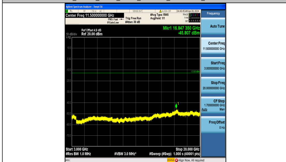
Band4_20MHz_QPSK_20175_100RB#0_3000~20000_3000~20000
