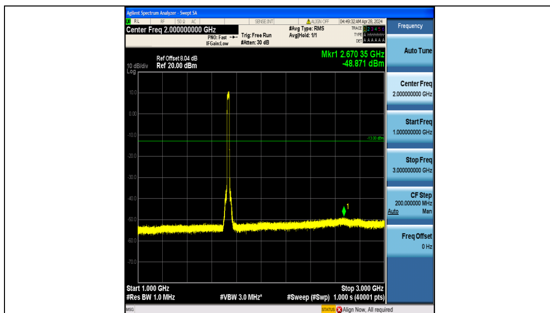
Band4_20MHz_QPSK_20175_100RB#0_1000~3000_1000~3000
