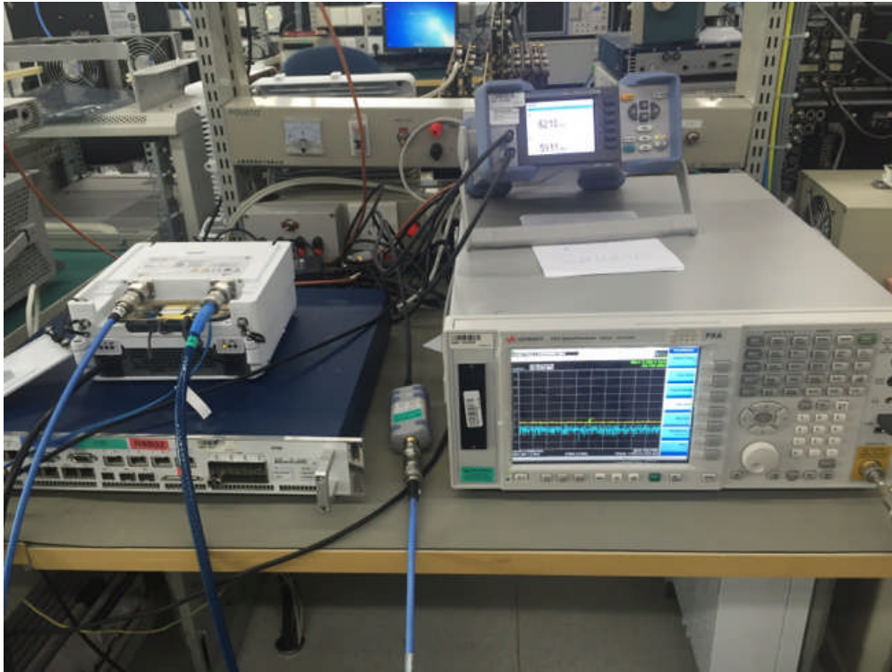
Conducted Testing Setup
