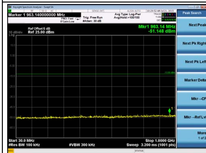
LTE band 7 - Middle CH 30MHz~1GHz 16QAM
