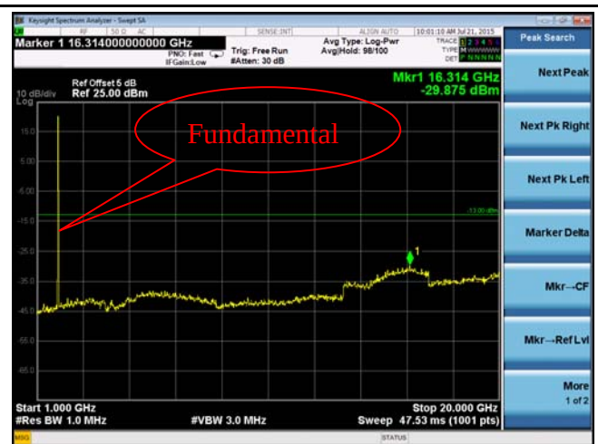
LTE band 2 - Middle CH Above 1GHz 16QAM
