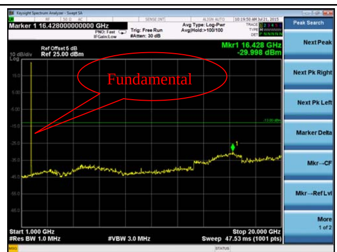
LTE band 4 - Middle CH Above 1GHz QPSK
