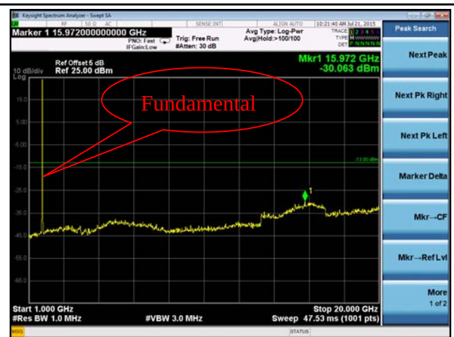
LTE band 4 - High CH Above 1GHz 16QAM
