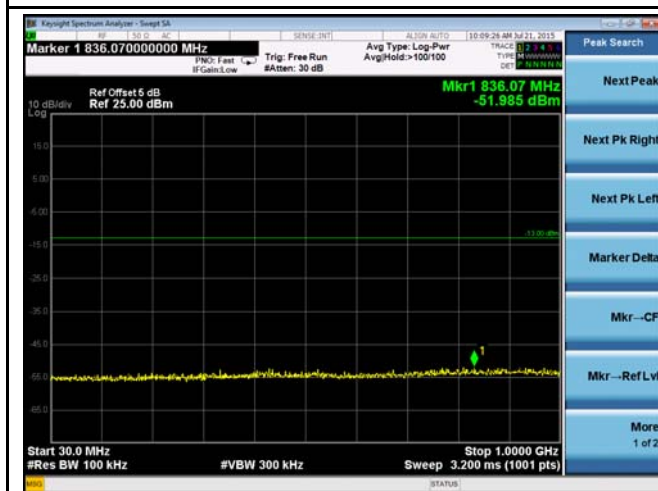
LTE band 2 - High CH 30MHz~1GHz QPSK
