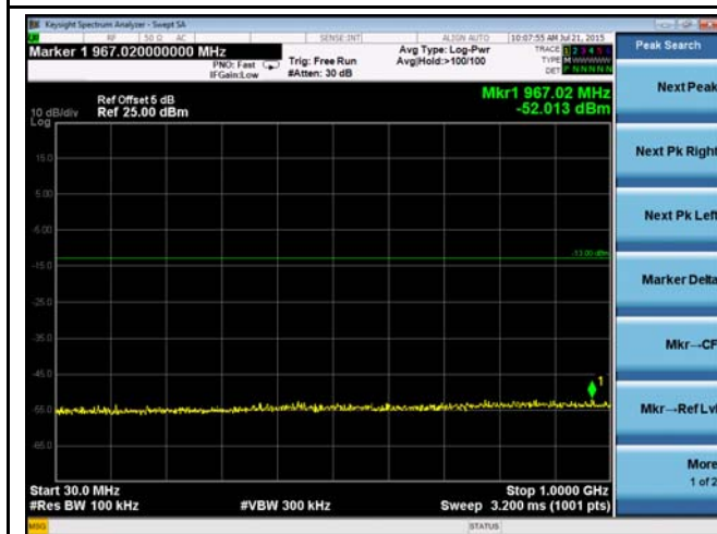
LTE band 2 - Middle CH 30MHz~1GHz 16QAM
