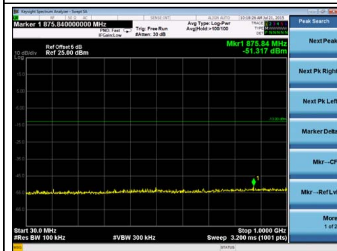
LTE band 4 - Middle CH 30MHz~1GHz 16QAM
