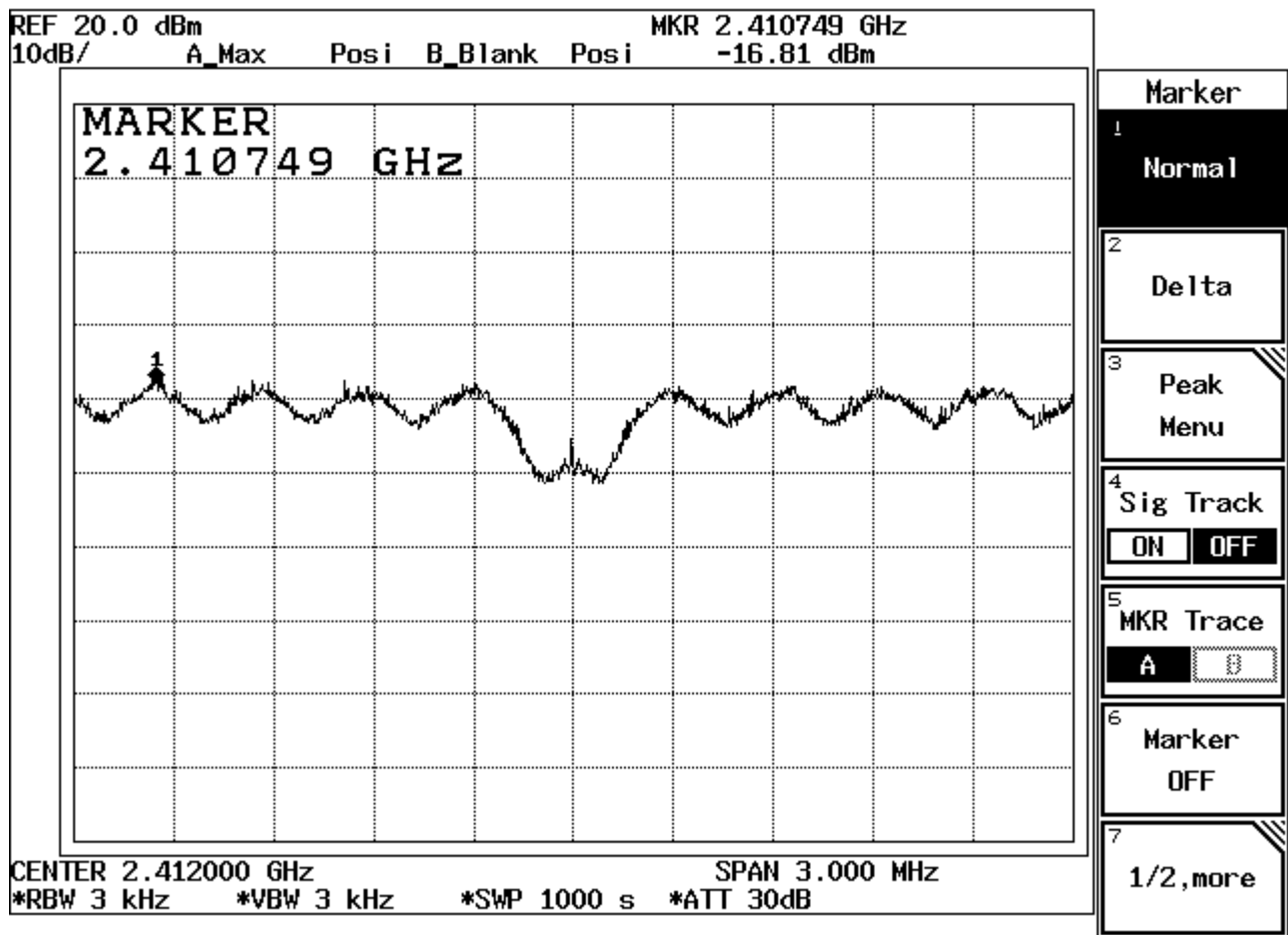
Figure Channel 1:
