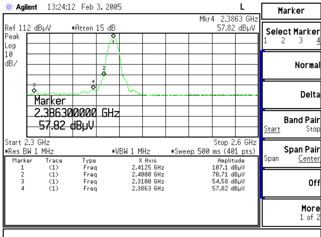
Figure Channel 1: (Horizontal)
