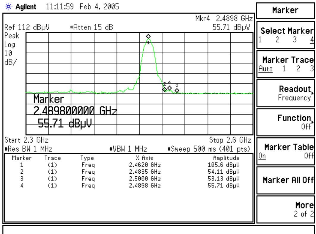
Figure Channel 11: (Horizontal)
