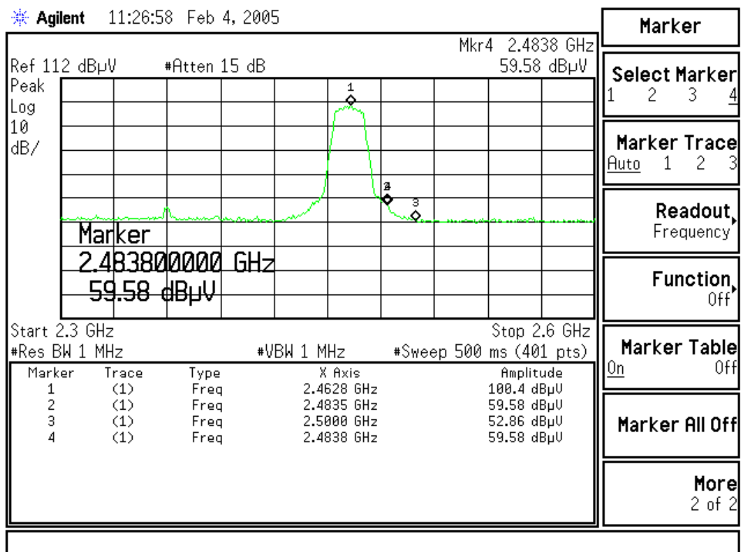
Figure Channel 11: (Vertical)
