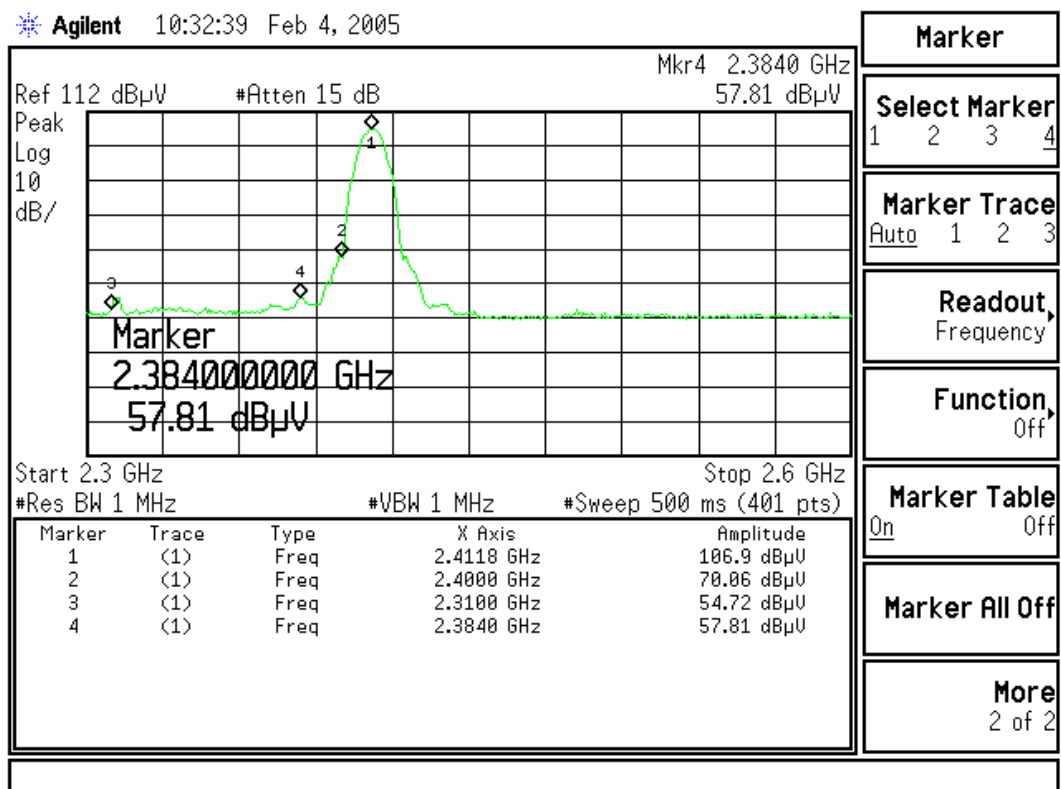
Figure Channel 1: (Vertical)
