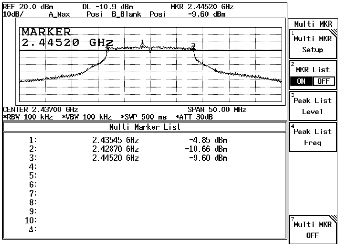
Figure Channel 6:
