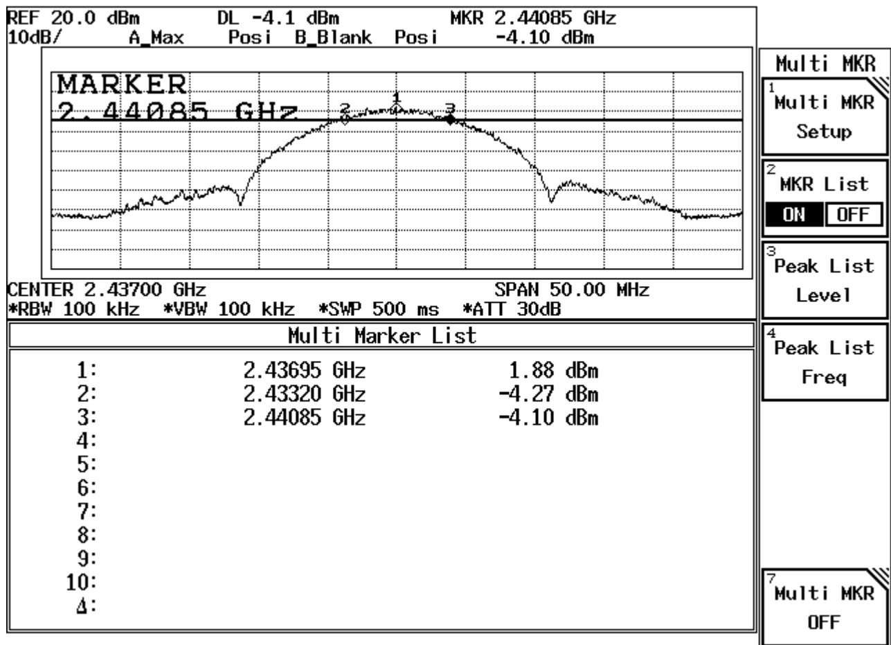
Figure Channel 6: 11Mbps
