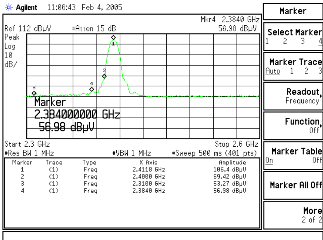
Figure Channel 1: (Horizontal)
