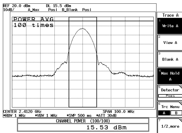
11Mbps-Ch01
