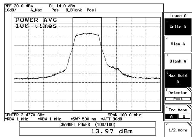
54Mbps-Ch06
