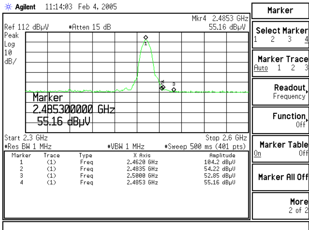
Figure Channel 11: (Vertical)
