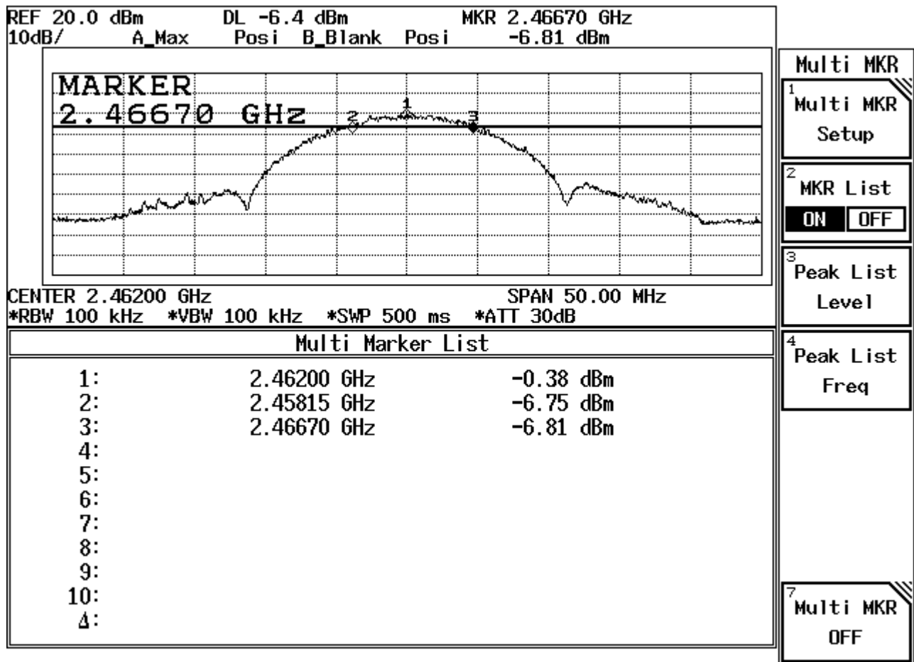
Figure Channel 11: 11Mbps
