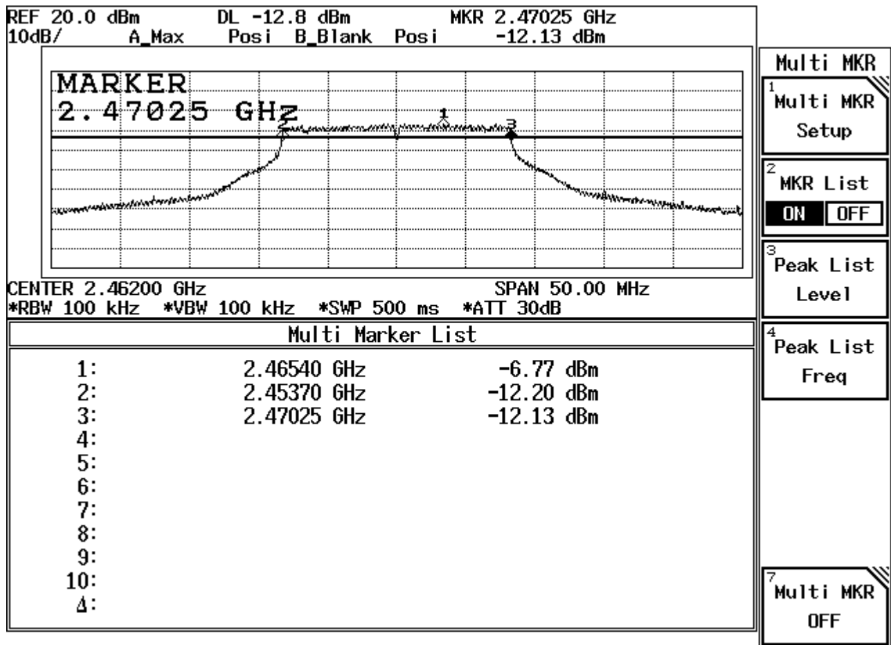
Figure Channel 11: 54Mbps
