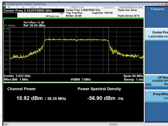
11AX40SISO-Ant1-2452-PASS
