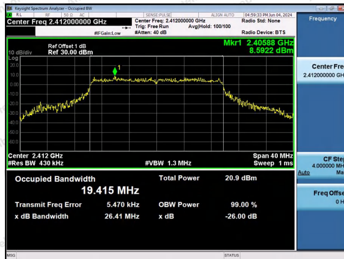
11AX20SISO-Ant1-2412
