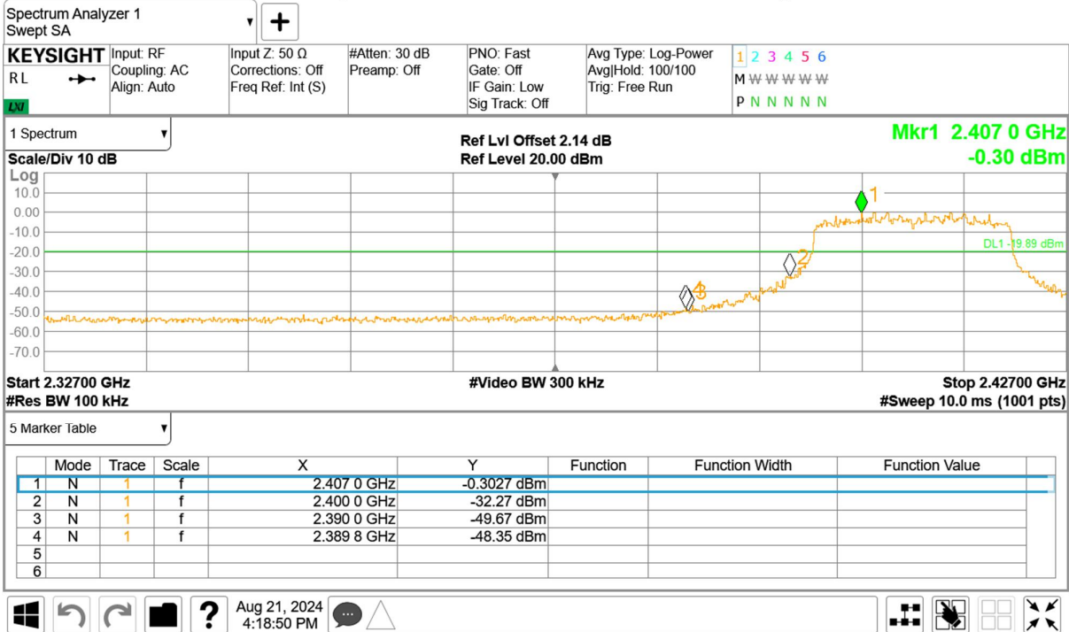
Band Edge NVNT ax20 2412MHz Ant1 Emission RU242_61
