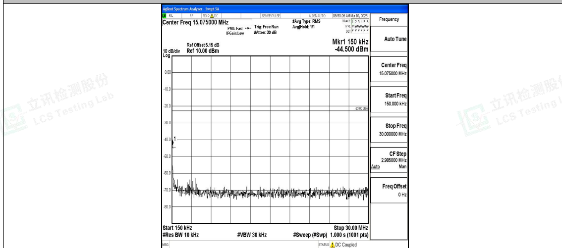
Band12_5MHz_16QAM_23095_1RB#0_0.15~30_0.15~30
