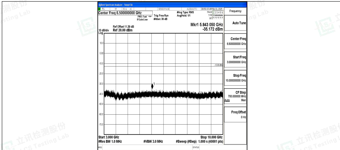
Band12_5MHz_QPSK_23095_1RB#0_3000~10000_3000~10000
