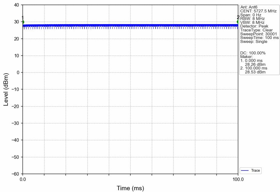
3M_LCH_5727.5MHz_Ant6_NTNV
