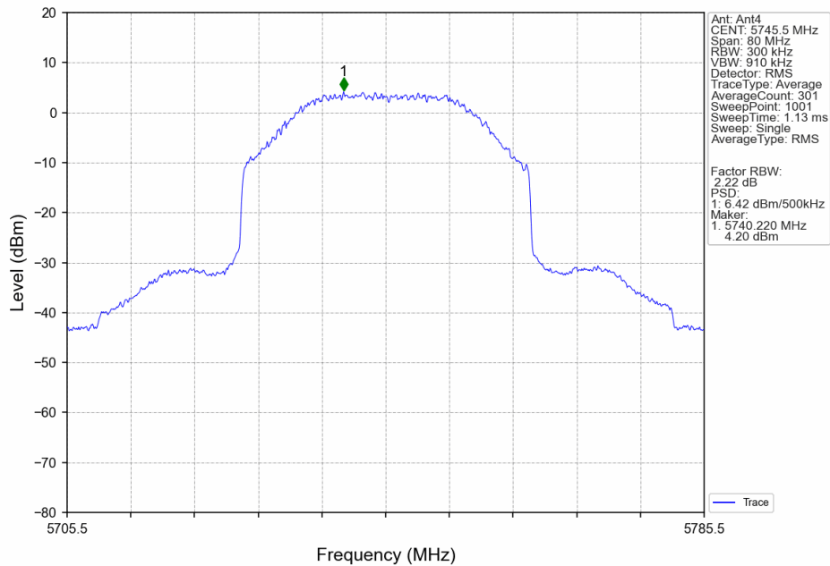
40M_LCH_5745.5MHz_Ant4_NTNV
