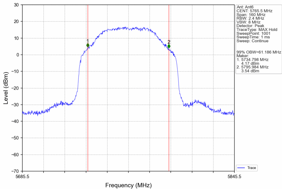
80M_LCH_5765.5MHz_Ant6_NTNV
