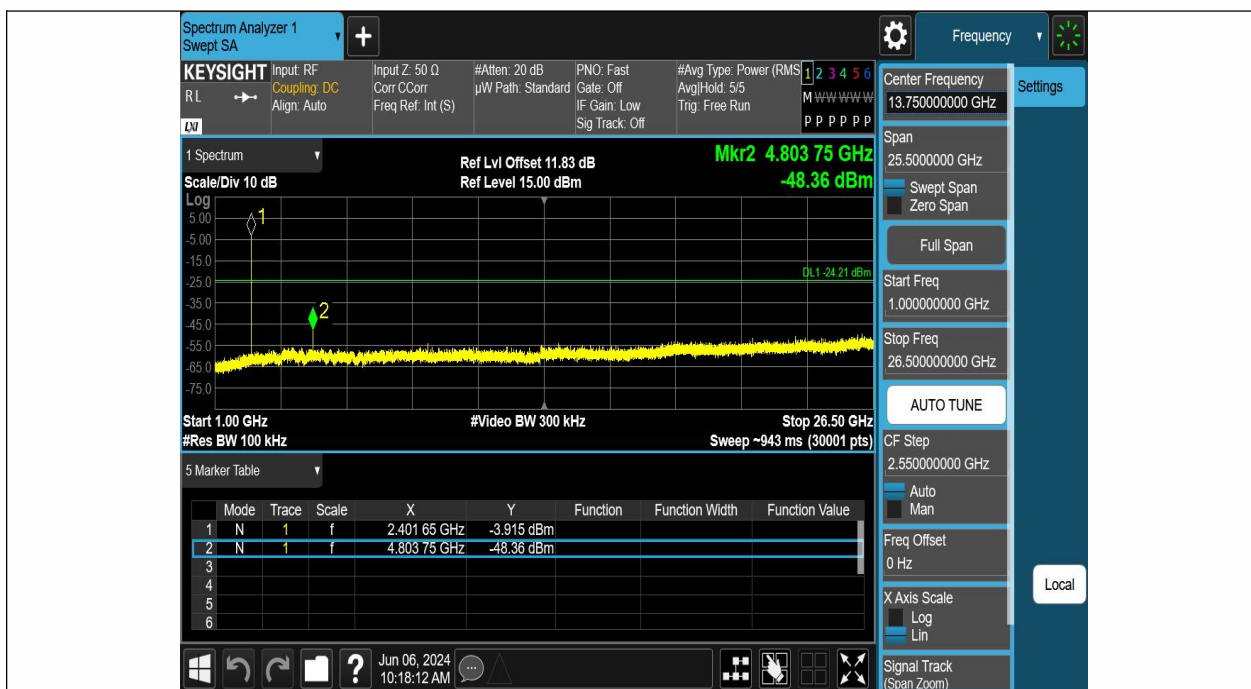
2.4G_1M-Ant1-2402-1000~26500-PASS
