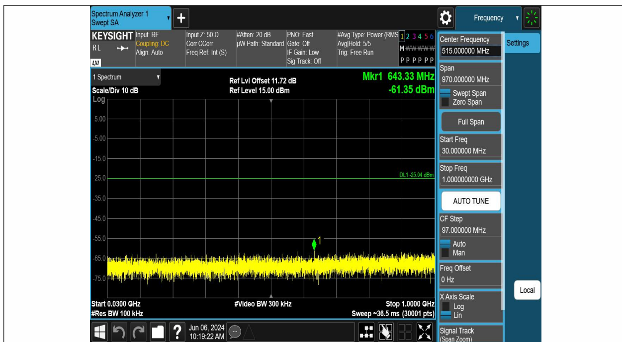
2.4G_1M-Ant1-2440-30~1000-PASS
