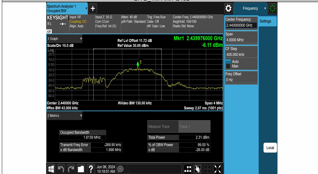
2.4G_1M-Ant1-2440
