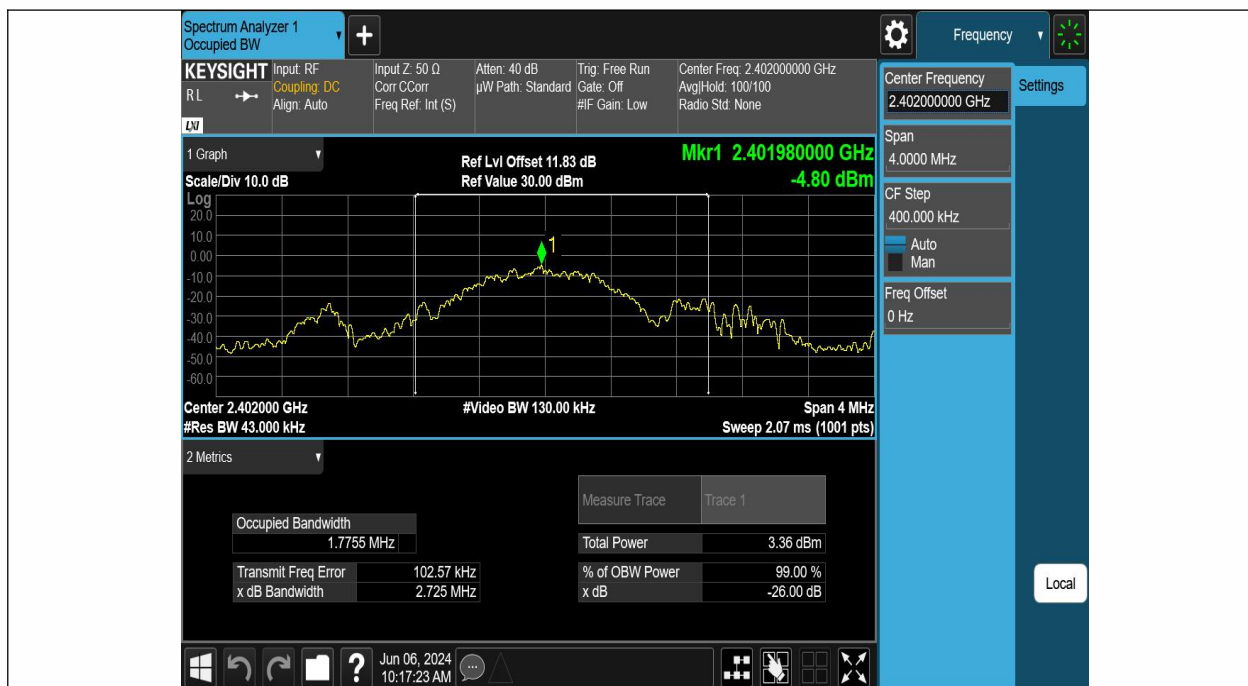
2.4G_1M-Ant1-2402
