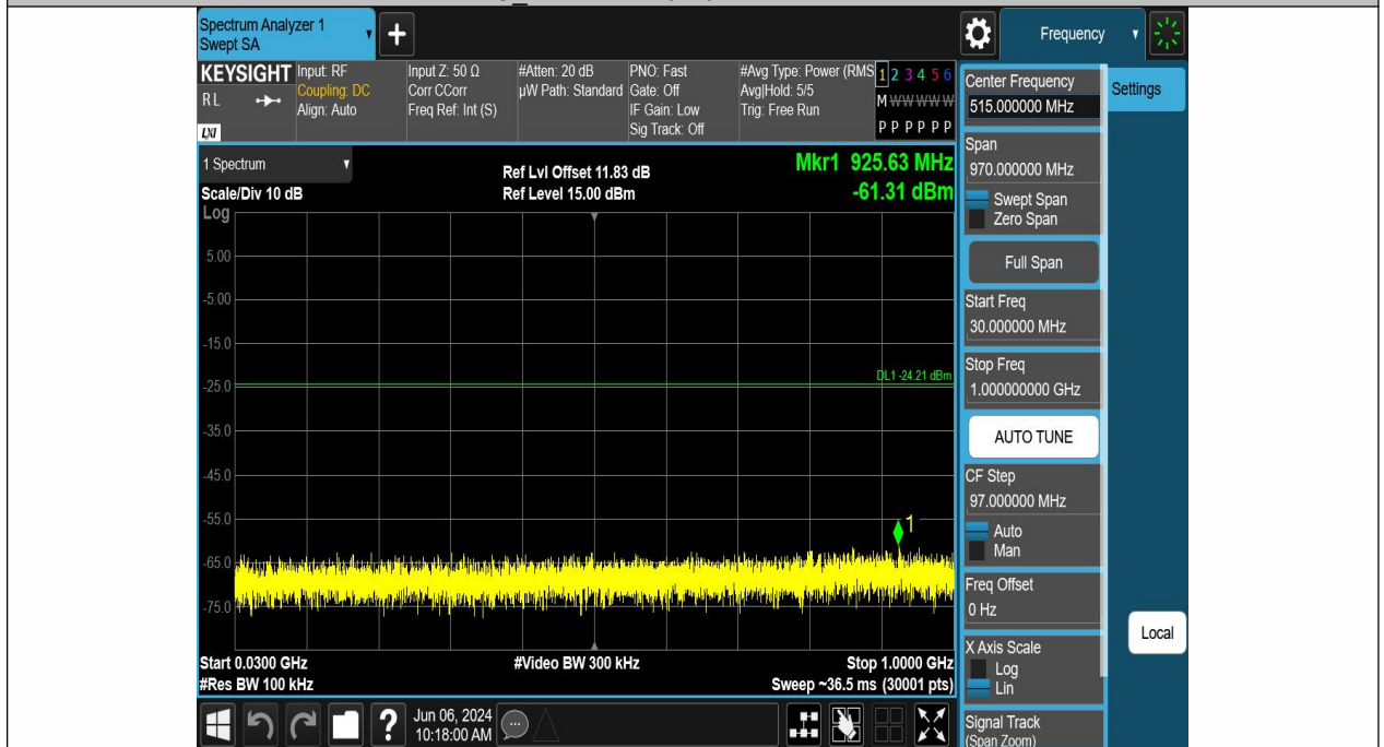
2.4G_1M-Ant1-2402-30~1000-PASS
