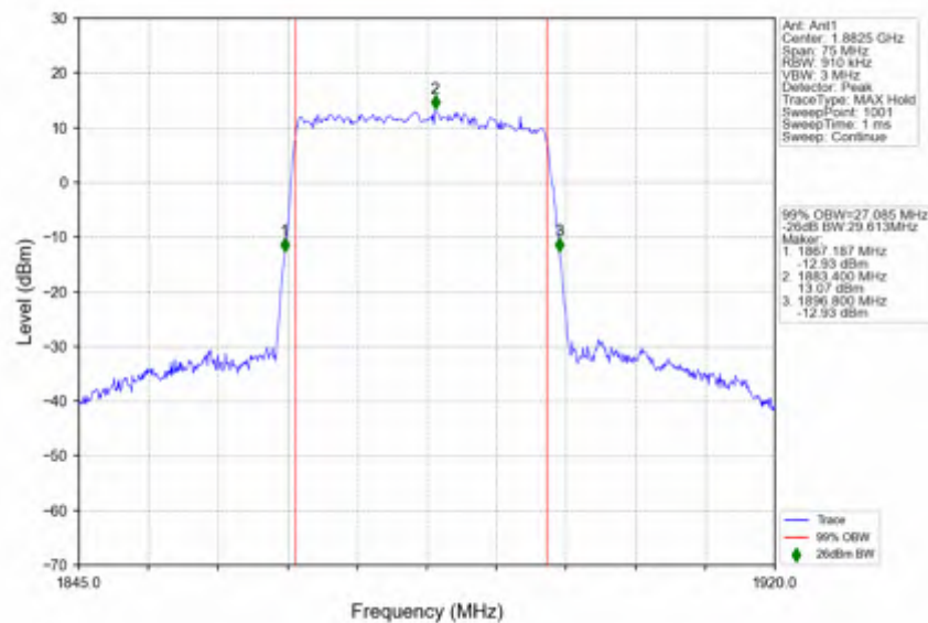
n25_30kHz_SISO_NTNV_30MHz_DFT-s-OFDM_QPSK_1900MHz_Outer_Full
