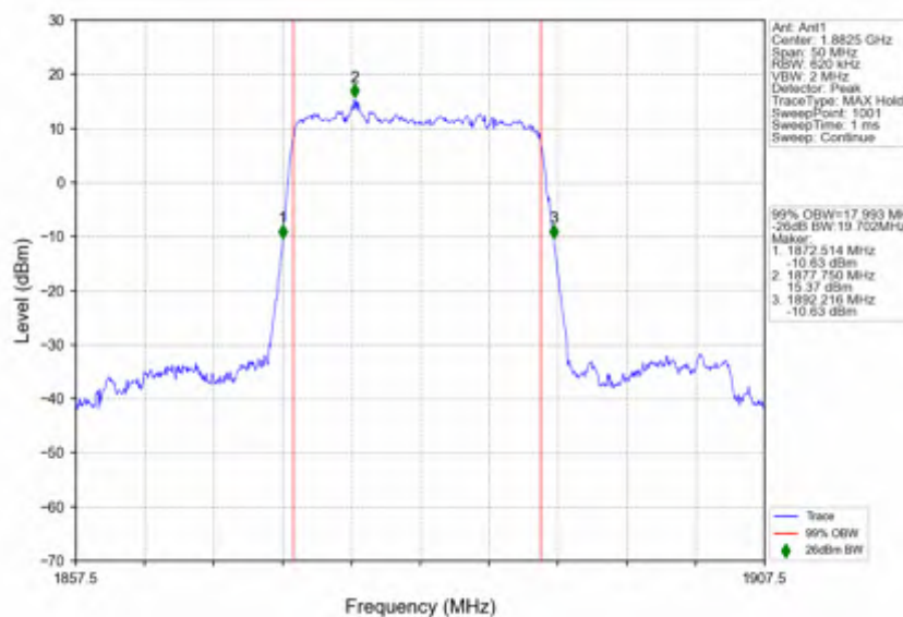
n25_30kHz_SISO_NTNV_20MHz_DFT-s-OFDM_PI/2_BPSK_1882.5MHz_Outer_Full
