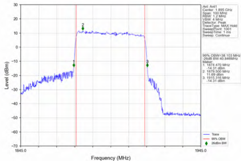
n25_30kHz_SISO_NTNV_40MHz_CP-OFDM QPSK_1895MHz_Outer_Full
