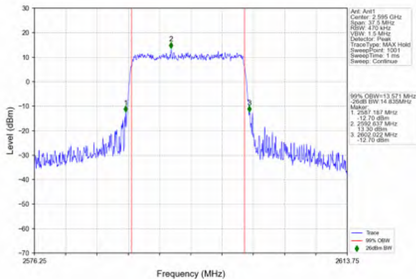
n38 15kHz SISO NTNv 15MHz DFT-s-OFDM 16 QAM 2595MHz Outer Full
