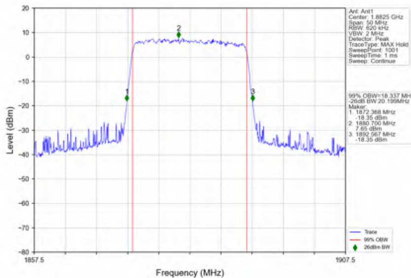
n25 30kHz SISO NTVN 20MHz CP-OFDM 256 QAM 1882.5MHz Outer Full
