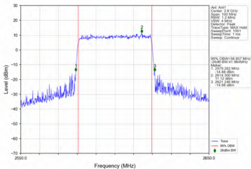
n38 15kHz SISO NTN 40MHz CP-OFDM 64 QAM 2600MHz Outer Full
