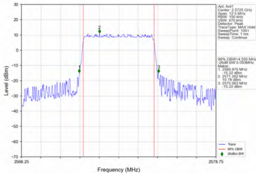
n38_15kHz_SISO_NTNV_5MHz_DFT-s-OFDM_64_QAM_2572.5MHz_Outer_Full
