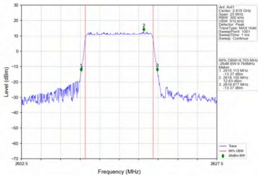
n38_30kHz_SISO_NTNV_10MHz_DFT-s-OFDM QPSK_2615MHz_Outer_Full
