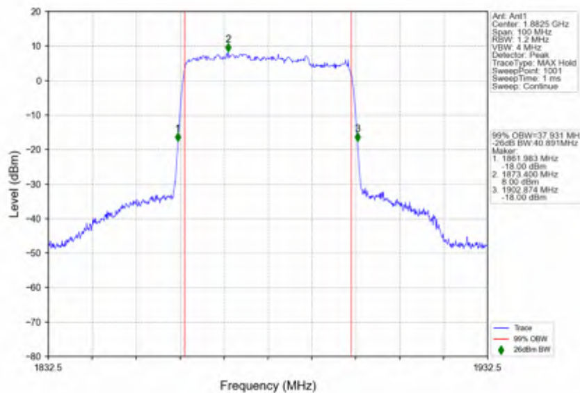
n25 30kHz SISO NTV 40MHz CP-OFDM 256 QAM 1882.5MHz Outer Full
