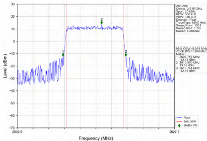
n38 15kHz SISO NTV 10MHz DFT-s-OFDM QPSK 2615MHz Outer Full
