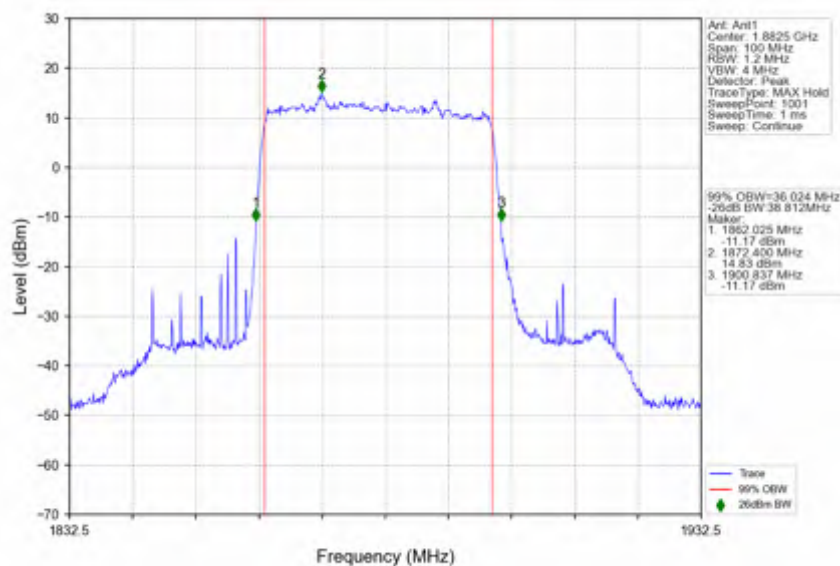
n25_30kHz_SISO_NTNV_40MHz_DFT-s-OFDM_PI/2_BPSK_1882.5MHz_Outer_Full
