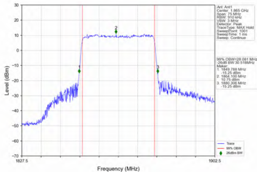
n25_30kHz_SISO_NTNV_30MHz_CP-OFDM 64 QAM_1865MHz_Outer_Full
