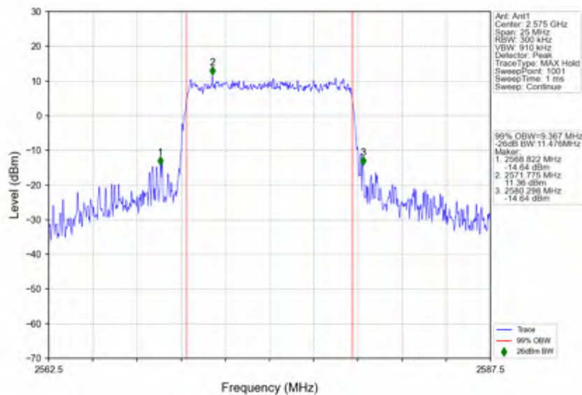
n38_15kHz_SISO_NTNV_10MHz_CP-OFDM QPSK_2575MHz_Outer_Full
