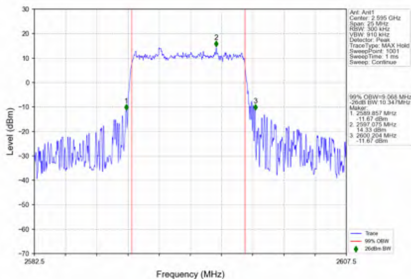
n38_15kHz_SISO_NTNV_10MHz_DFT-s-OFDM_PI/2_BPSK_2595MHz_Outer_Full
