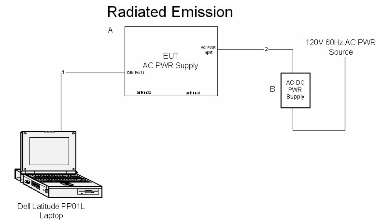
Figure 2. Block Diagram of Test Configuration (Radiated Emissions)
