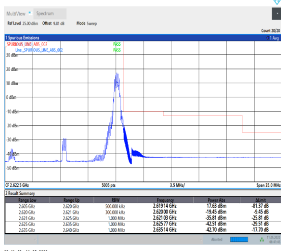
1-N38-PC2-30-15-H-5-CP-QPSK-Edge_1RB_Right-1@37-Ant0-PASS-see graph
