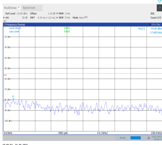
1-N38--30-40-M-1-DFT-PI2BPSK-Inner_1RB_Left-1 @1-0.009-0.15-Ant0--79.96--55-PASS
