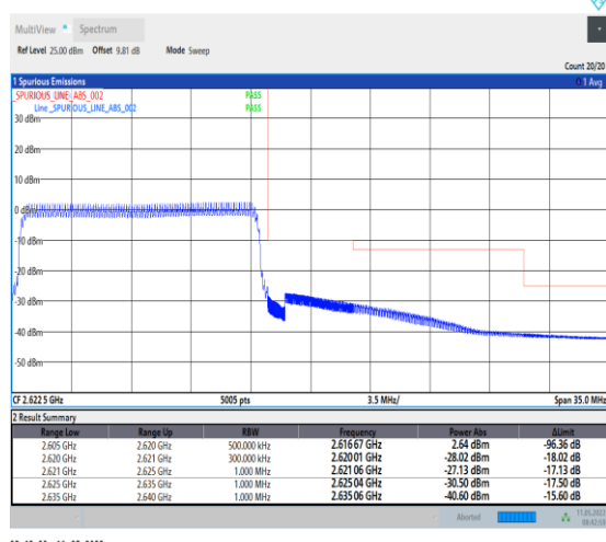
1-N38-PC2-30-15-H-6-CP-QPSK-Outer_Full-38@0-Ant0-PASS-see graph
