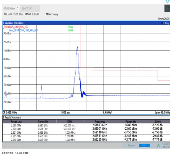
1-N38-PC2-30-30-H-5-CP-QPSK-Edge_1RB_Right-1@ 77-Ant0-PASS-see graph
