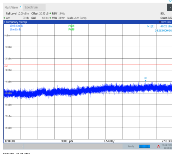
1-N38--30-40-L-1-DFT-PI2BPSK-Inner_1RB_Left-1@ 1-12000-27000-Ant0--40.23--25-PASS
