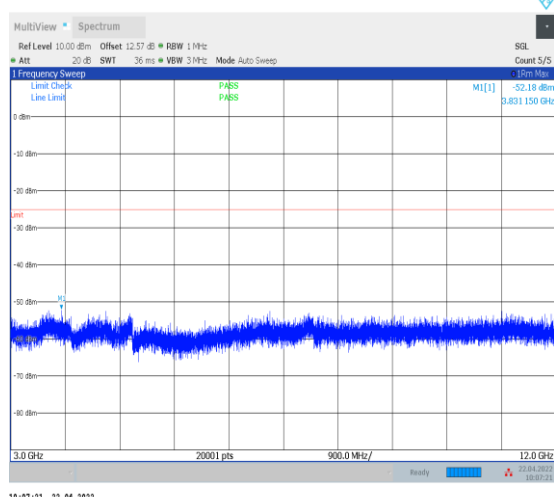
1-N38--30-40-M-1-DFT-PI2BPSK-Inner_1RB_Left-1 @1-3000-12000-Ant0--52.18--25-PASS
