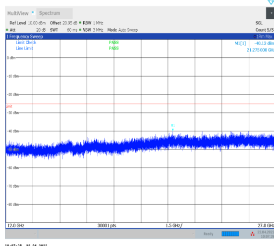
1-N38--30-40-M-1-DFT-PI2BPSK-Inner_1RB_Left-1 @1-12000-27000-Ant0--40.13--25-PASS
