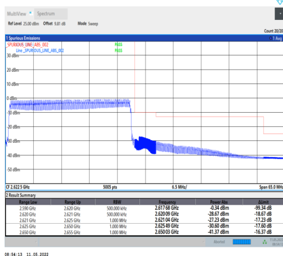
1-N38-PC2-30-30-H-6-CP-QPSK-Outer_Full-78@ 0-Ant0-PASS-see graph
