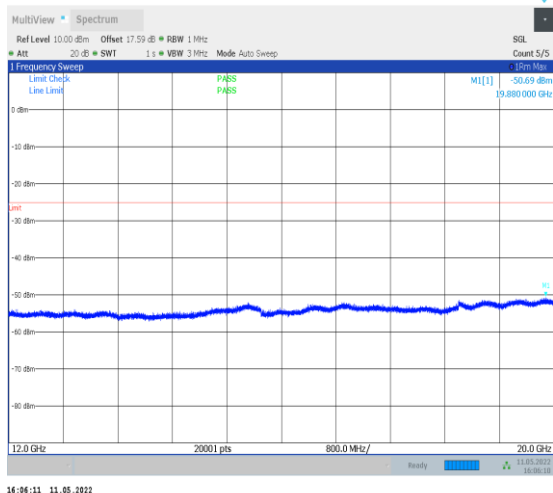
1-N38-PC2-30-40-H-1-DFT-QPSK-Edge_1RB_Left-1 @0-12000-20000-Ant0--50.69--25-PASS
