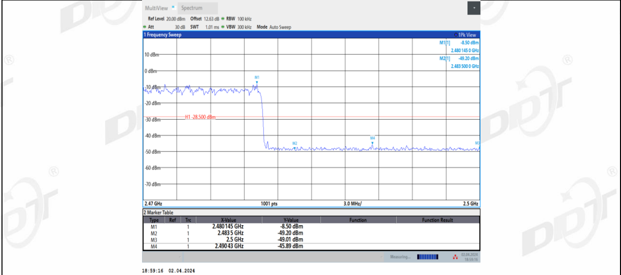
2DH5_Right side_High_Hop_2480
