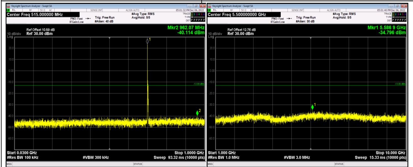
Band17-5MHz-QPSK-23825-1RB#0-Range1:30~1000MHz
