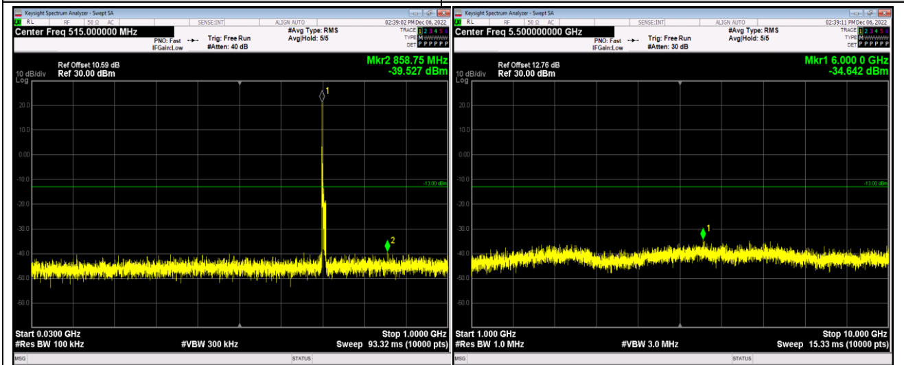
Band12-10MHz-64QAM-23060-1RB#0-Range1:30 ~1000MHz
