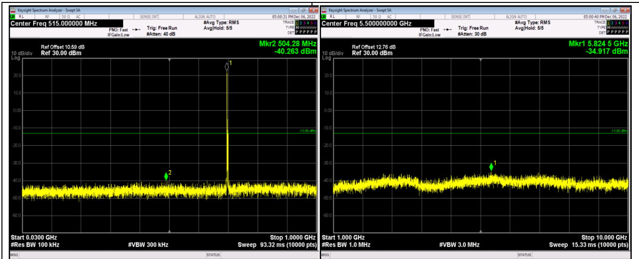
Band17-5MHz-QPSK-23790-1RB#0-Range1:30~1000MHz
