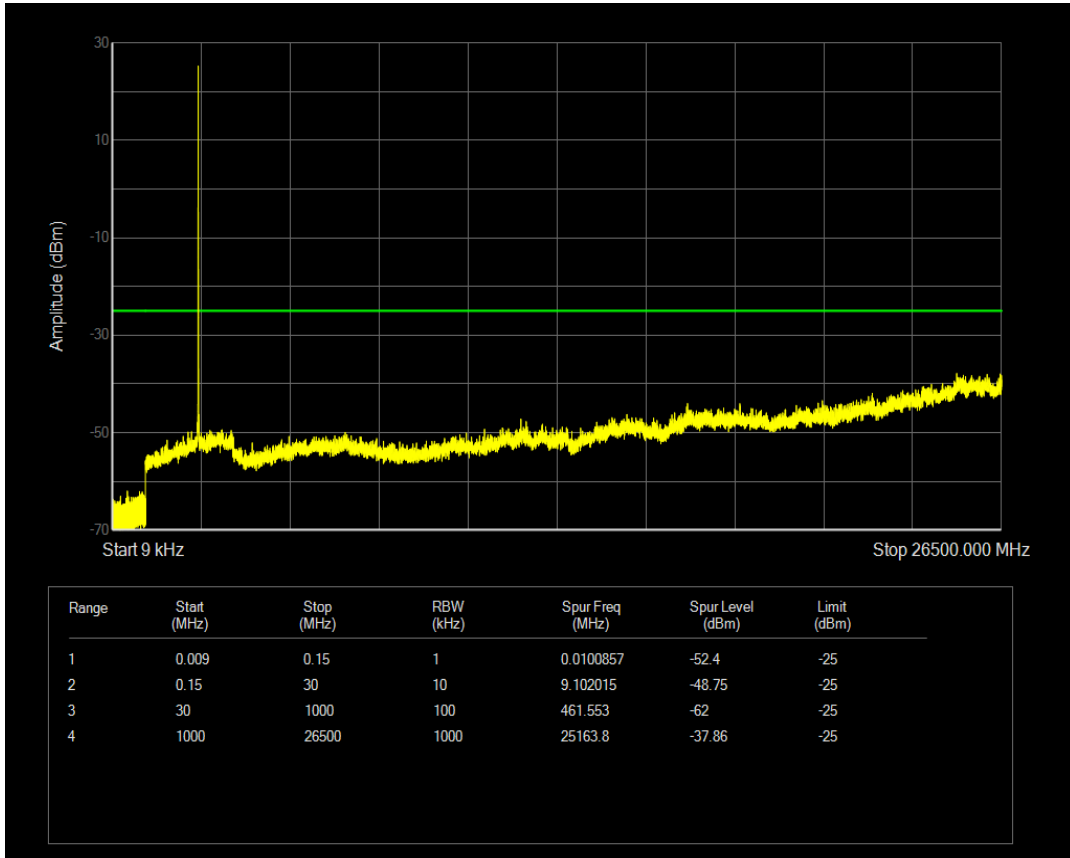
Band41 16QAM BW=5MHz Channel=40415 RB Size=25 Position=#0
