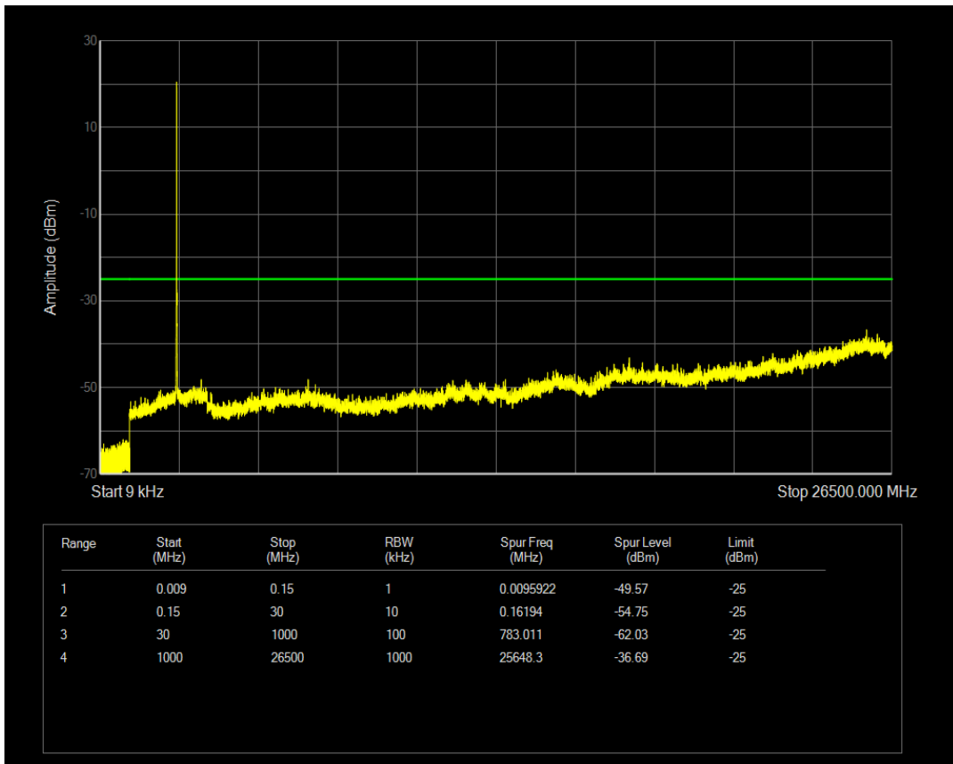
Band41 16QAM BW=5MHz Channel=40415 RB Size=1 Position=#0
