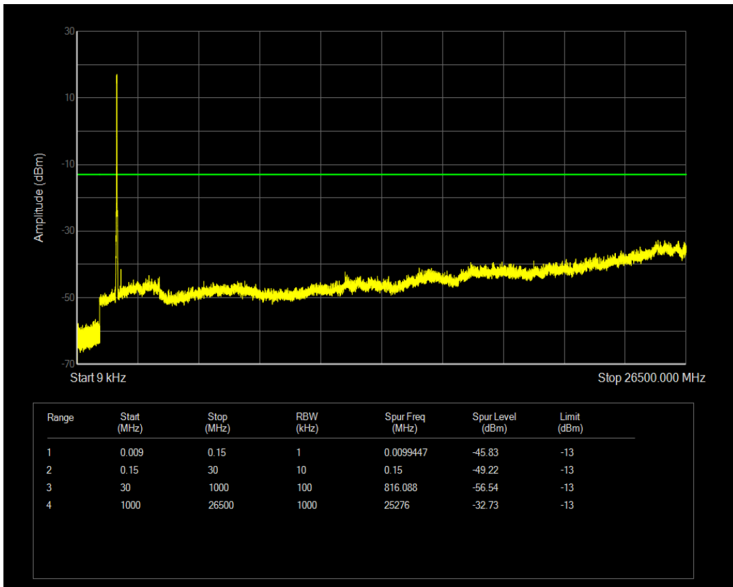
Band41 QPSK BW=5MHz Channel=40415 RB Size=1 Position=#0
