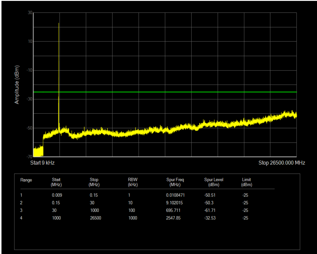
Band41 QPSK BW=5MHz Channel=40415 RB Size=25 Position=#0
