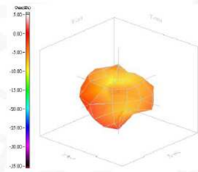
2.484GHz
