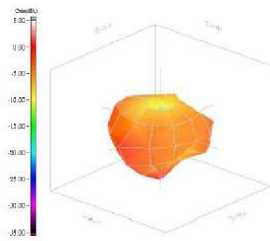
2.4GHz
