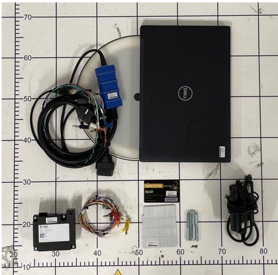
5. Front View of the DUT and accessories
