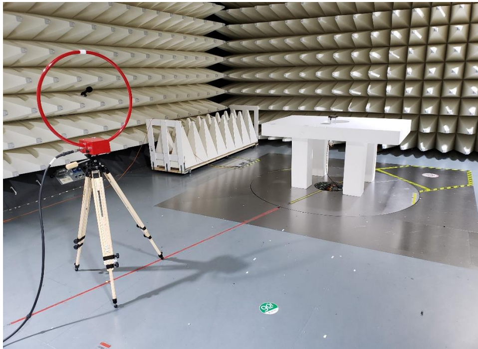
6. Low Range Radiated Emission test setup 9KHz to 30MHz
