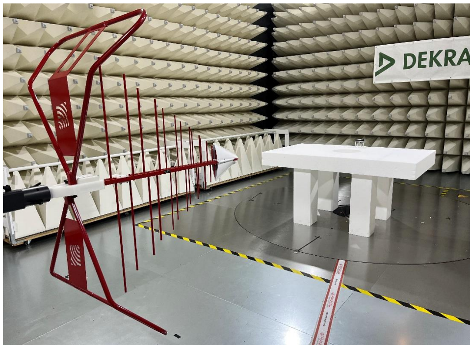
7. Low Range Radiated Emission test setup (30MHz to 1GHz)
