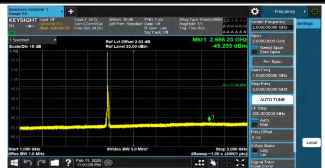
Band66-10MHz-QPSK-132622-1RB#0-1000~3000-PASS
