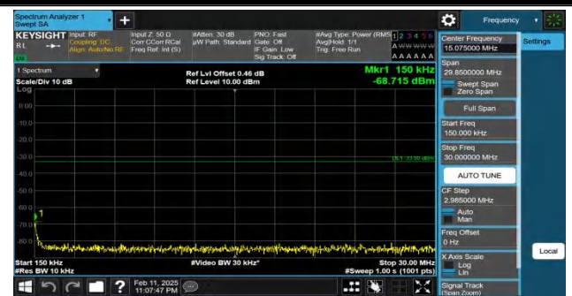
Band66-15MHz-QPSK-132047-1RB#0-0.15~30-PASS
