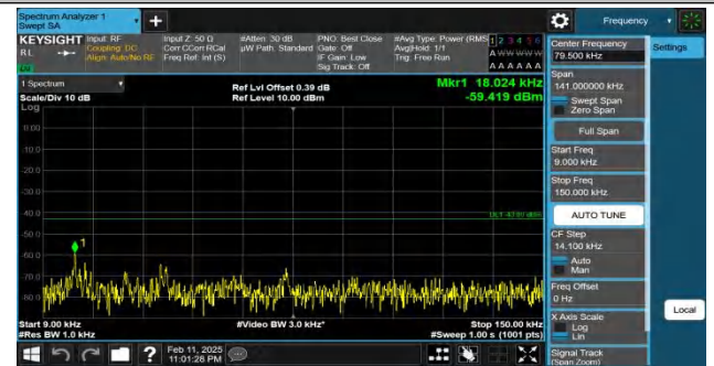
Band66-10MHz-QPSK-132622-1RB#49-0.009~0.15-PASS
