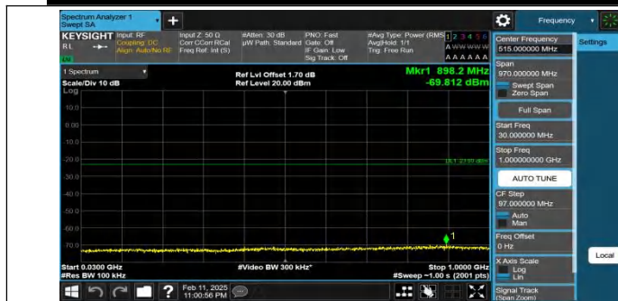
Band66-10MHz-QPSK-132622-1RB#0-30~1000-PASS
