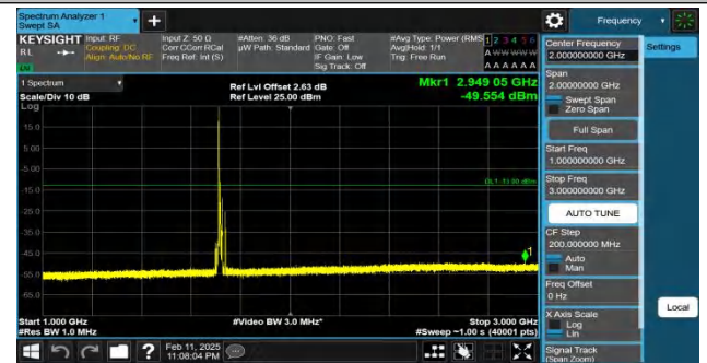
Band66-15MHz-QPSK-132047-1RB#0-1000~3000-PASS
