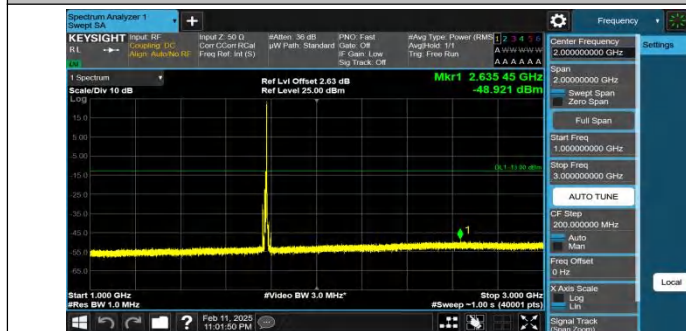
Band66-10MHz-QPSK-132622-1RB#49-1000~3000-PASS
