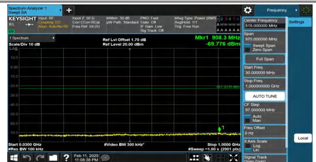
Band66-15MHz-QPSK-132047-1RB#74-30~1000-PASS
