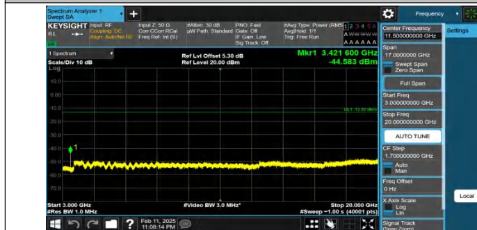
Band66-15MHz-QPSK-132047-1RB#0-3000~20000-PASS
