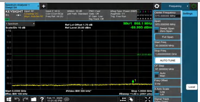
Band66-10MHz-QPSK-132622-1RB#49-30~1000-PASS
