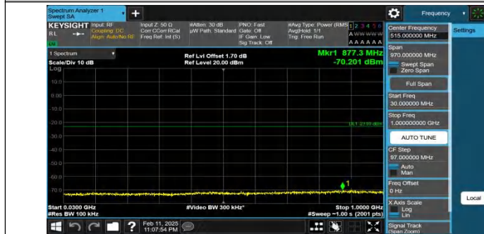
Band66-15MHz-QPSK-132047-1RB#0-30~1000-PASS
