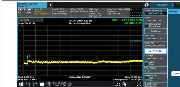
Band66-10MHz-QPSK-132622-1RB#0-3000~20000-PASS
