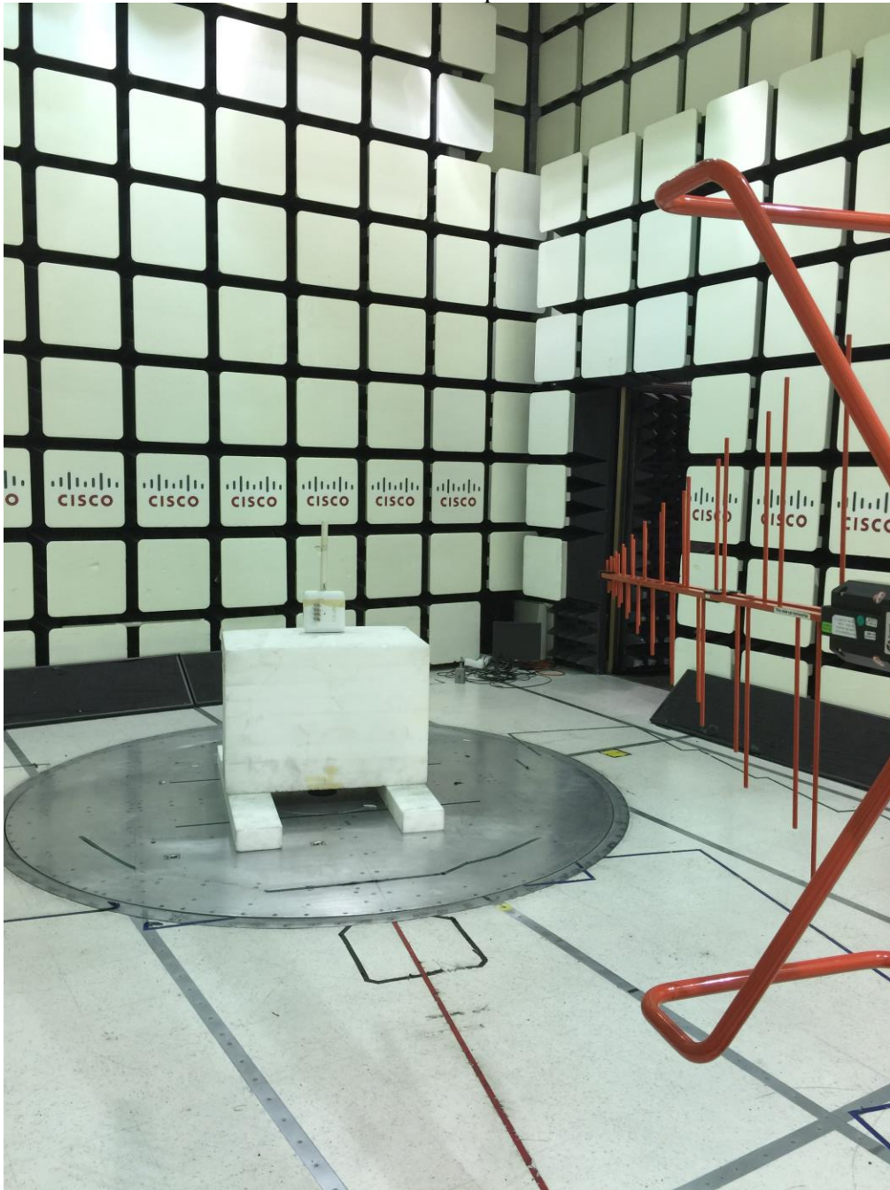
AIR-AP3802I-B-K9 Radiated Emissions setup 30MHz – 1GHz
