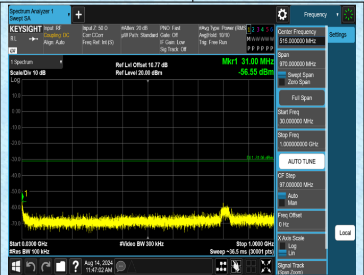
11N40SISO-Ant1-2437-30~1000
