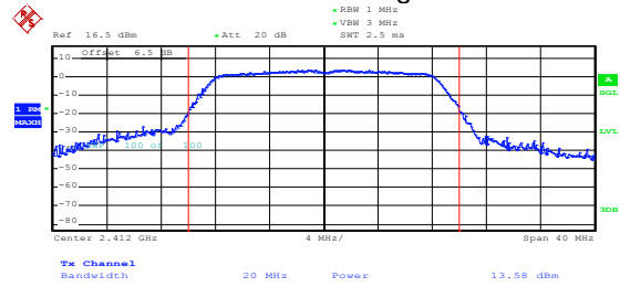
802.11g
