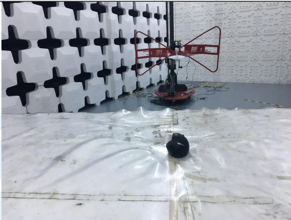
Radiated emission Test Setup (30 MHz~1 GHz)-Mouse
