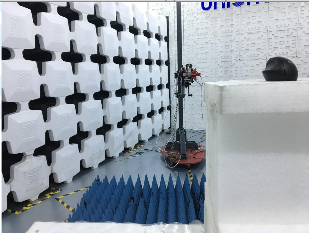
Radiated emission Test Setup (Above 1 GHz) -Mouse
