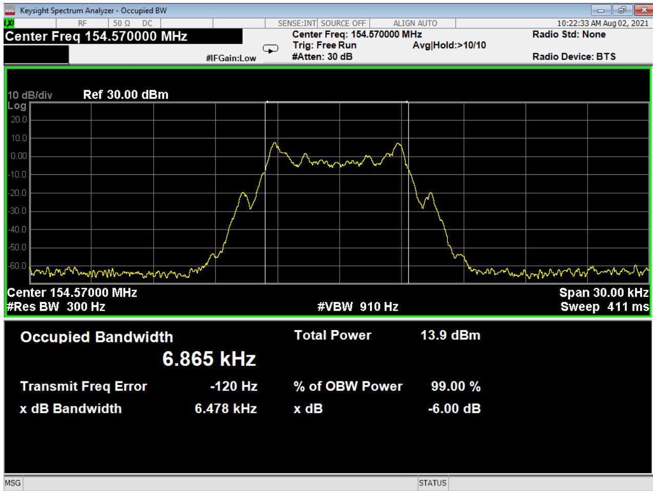
Figure 12 - Bandwidth, 154.570 MHz
