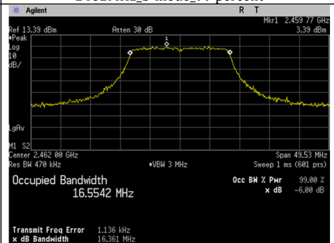
2462MHz_g-mode_99 percent
