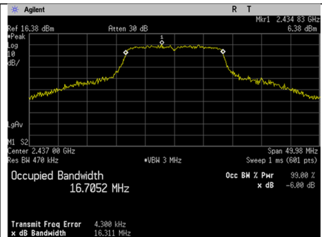
2437MHz_g-mode_99 percent
