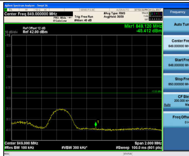
Band5_5MHz_QPSK_20625_25RB#0_-21.11_PASS
