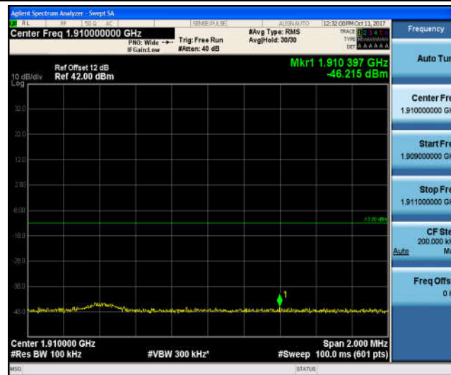
Band2_10MHz_QPSK_19150_50RB#0_-30.07_PASS
