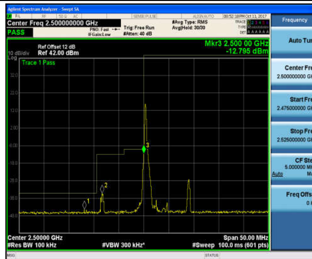
Band7_5MHz_QPSK_20775_25RB#0_-43.92,-28.43,-18.29_PASS
