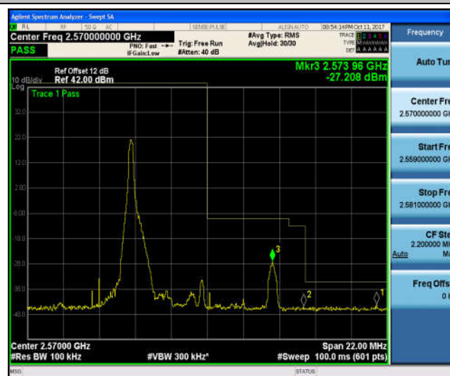
Band7_5MHz_QPSK_21425_25RB#0_-38.12,-37.57,-21.25_PASS
