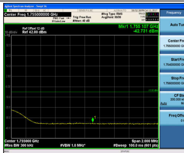
Band4_20MHz_QPSK_20300_100RB#0_-30.11_PASS
