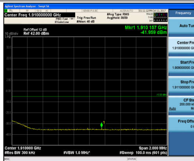
Band2_20MHz_16QAM_19100_1RB#0_-42.82_PASS
