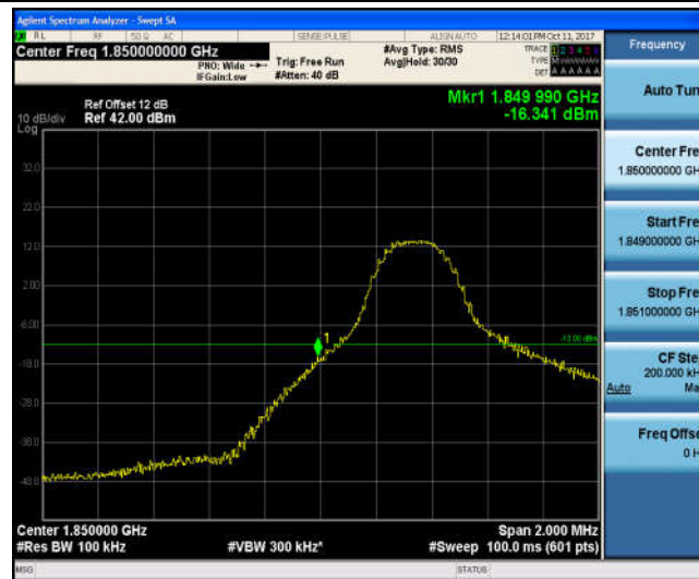
Band2_5MHz_QPSK_18625_25RB#0_-27.85_PASS
