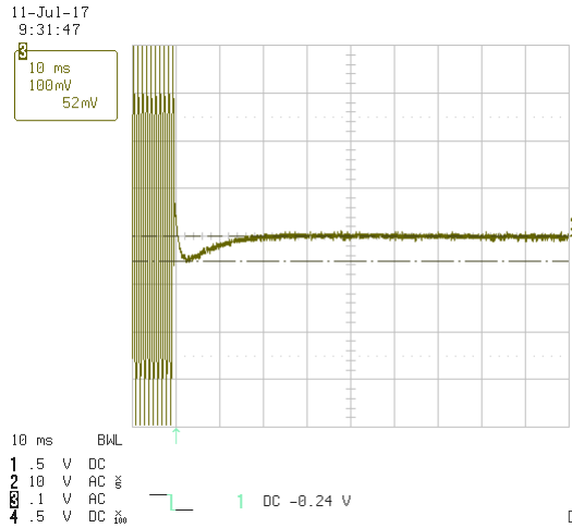
Plot 7.7.4 Transient frequency during power OFF test results at mid carrier frequency
