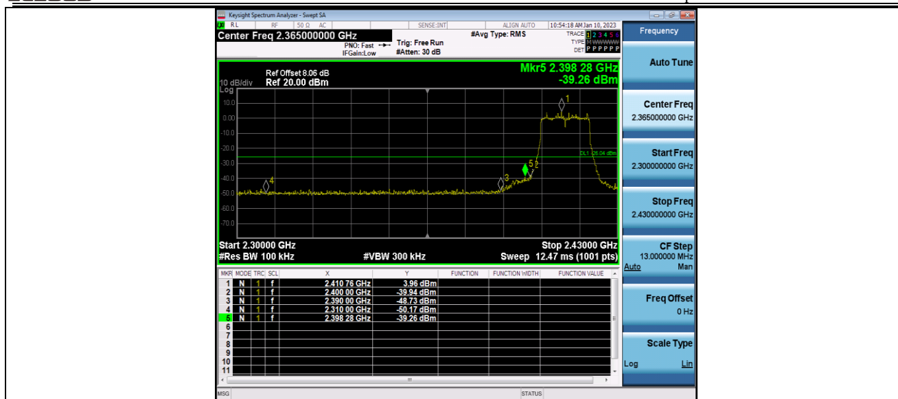
11G-CDD_Ant2_Low_2412
